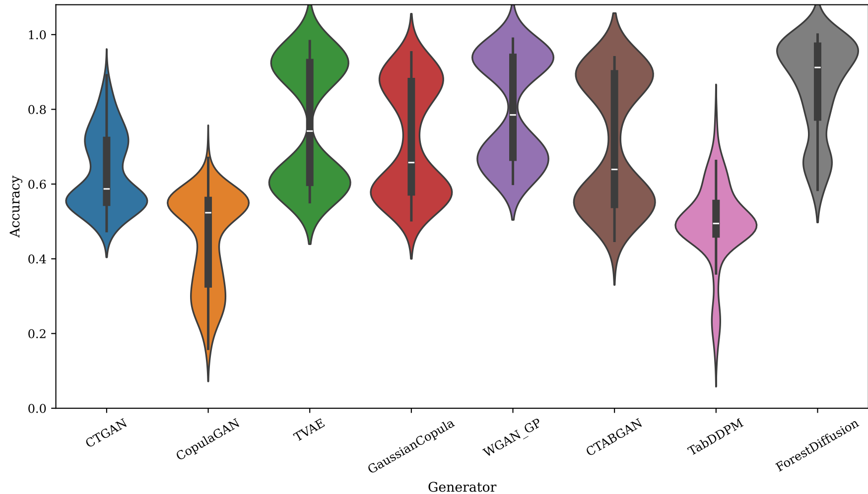
Violin Plots — Accuracy by Generator (approx. seed distribution)
