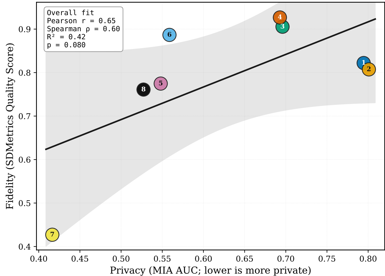
Fidelity vs Privacy (MIA AUC)
