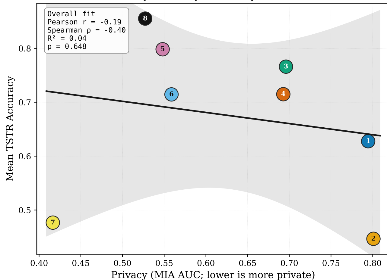
Privacy vs Utility (Accuracy, MIA AUC)
