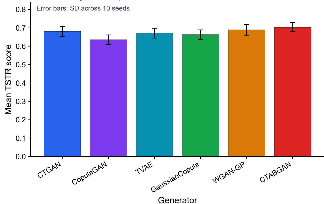
Average TSTR performance across datasets and classifiers
