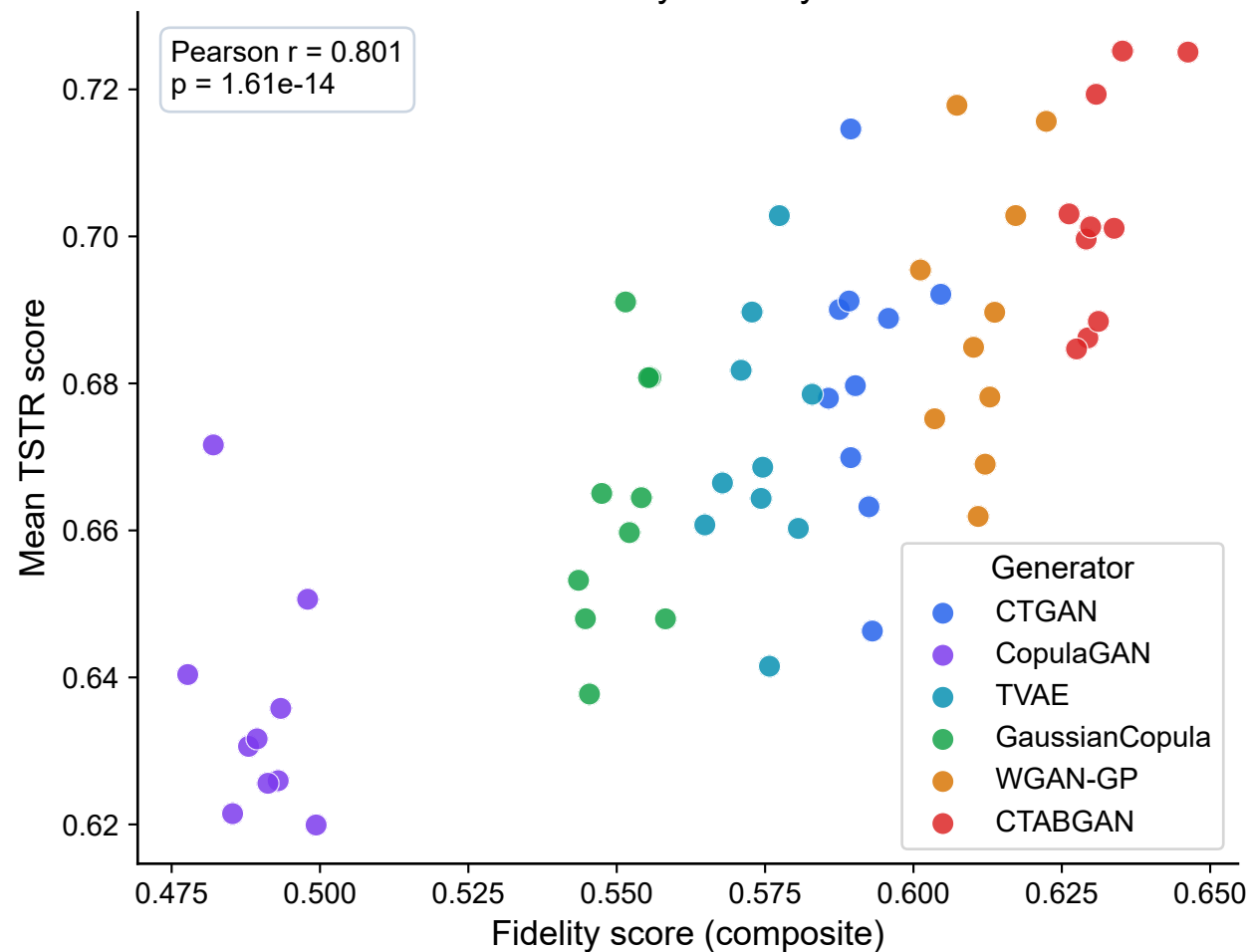
Fidelity vs utility
