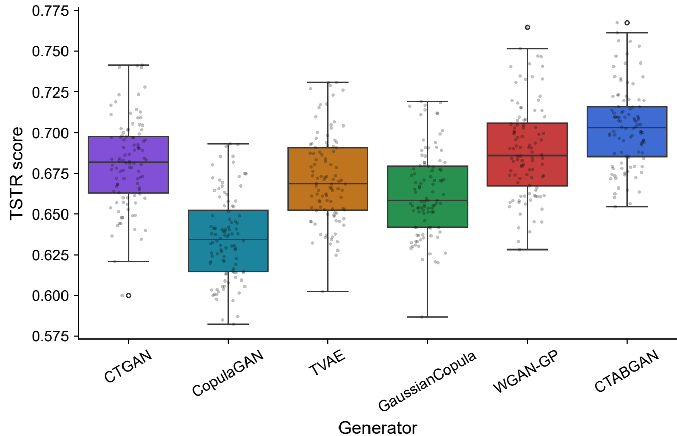
TSTR distribution across random seeds
