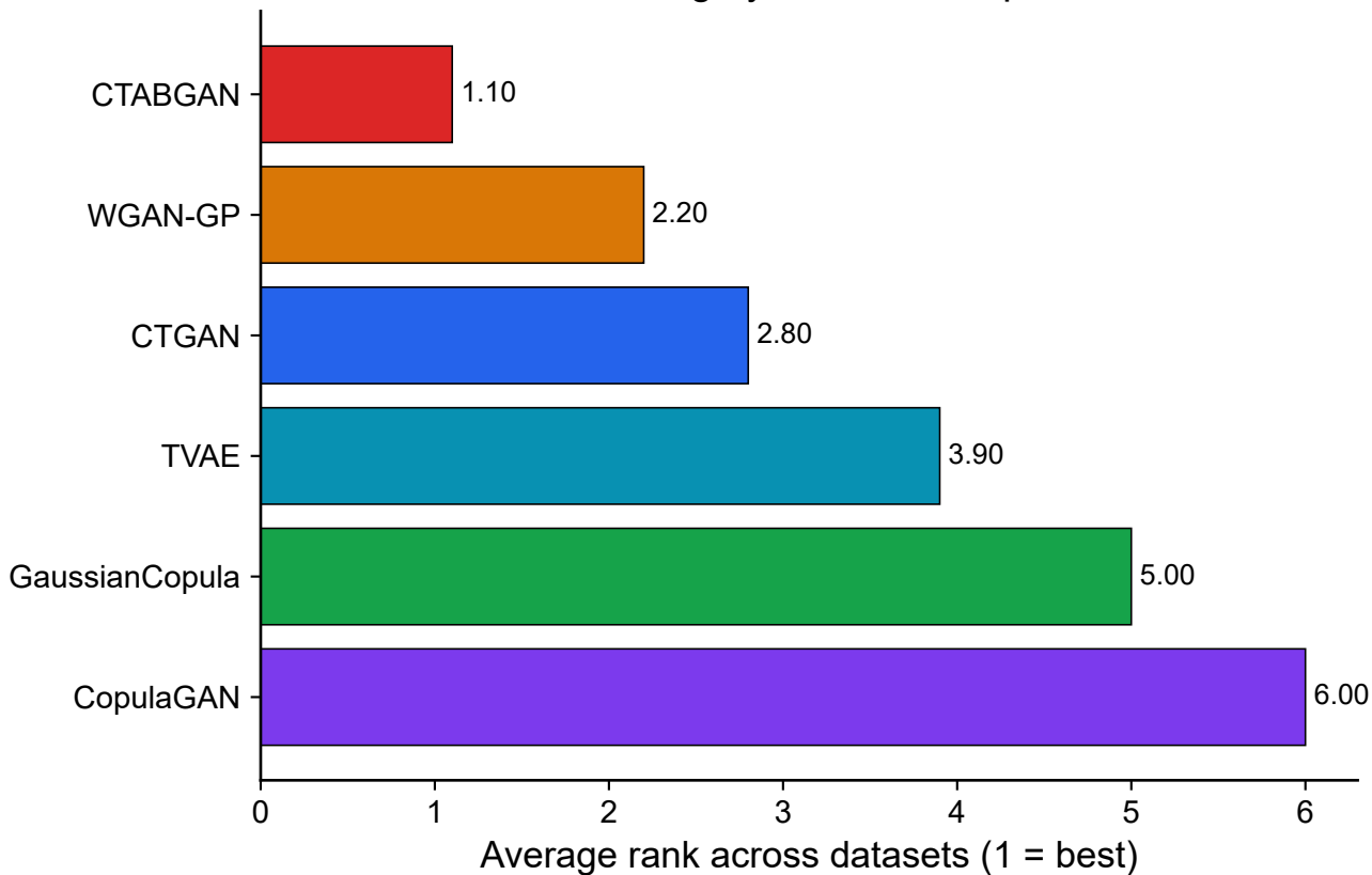
Generator ranking by mean TSTR performance
