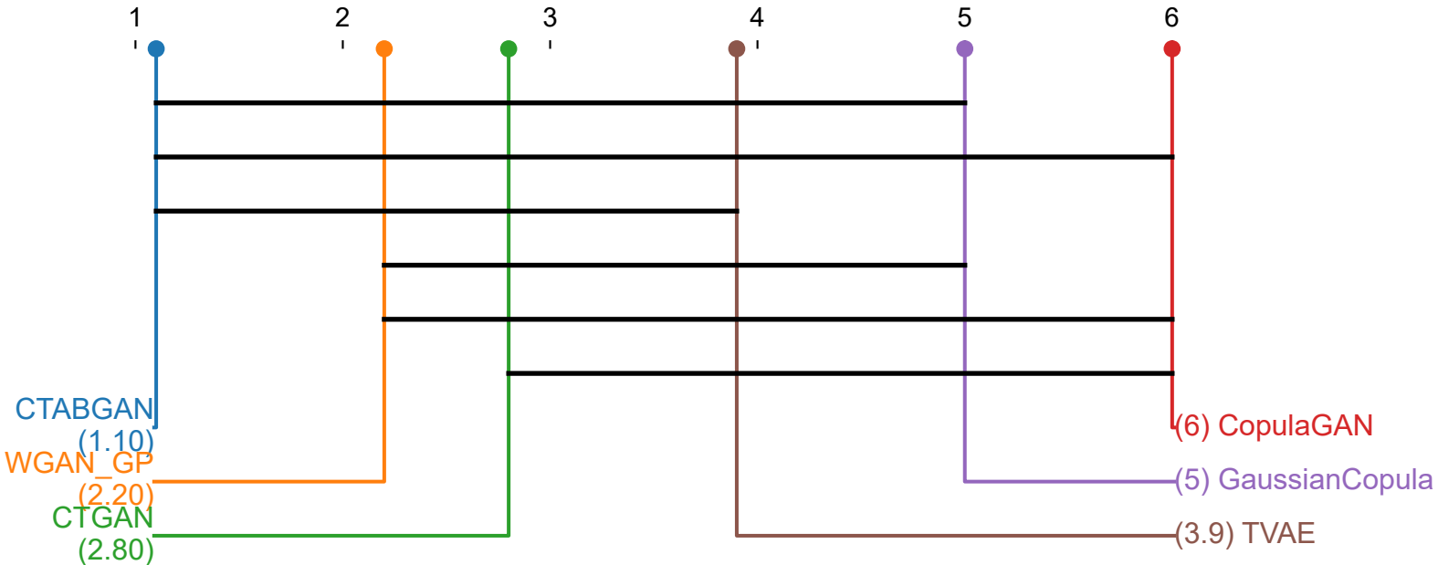
Critical difference diagram (Friedman \chi^2=47.43 , p=4.65e-09 )
