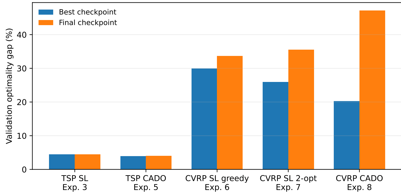
Paper-Selected Experiments: Best vs. Final Gap
