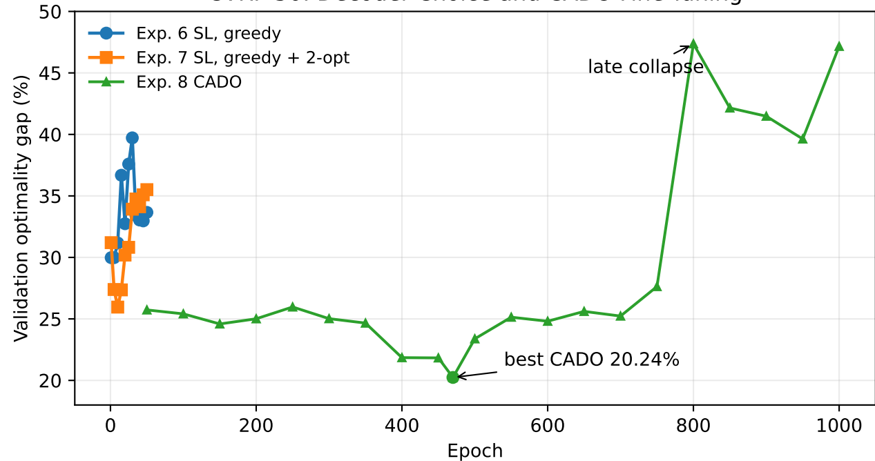
CVRP-50: Decoder Choice and CADO Fine-Tuning
