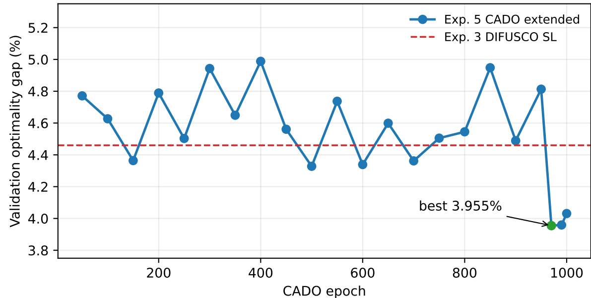
TSP-50: DIFUSCO SL vs. CADO Fine-Tuning
