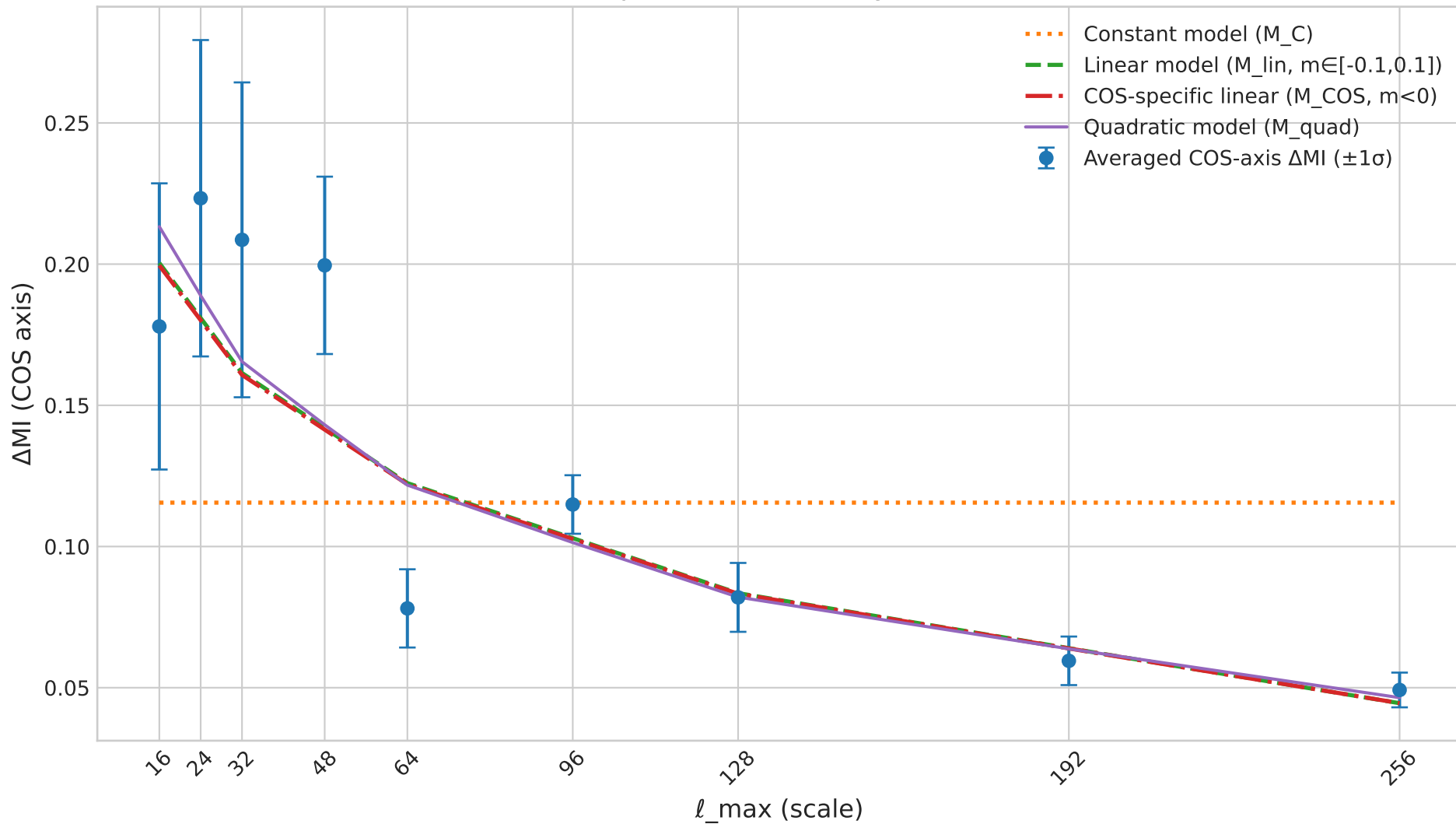
\Delta MI scale dependence and Bayesian model fits
