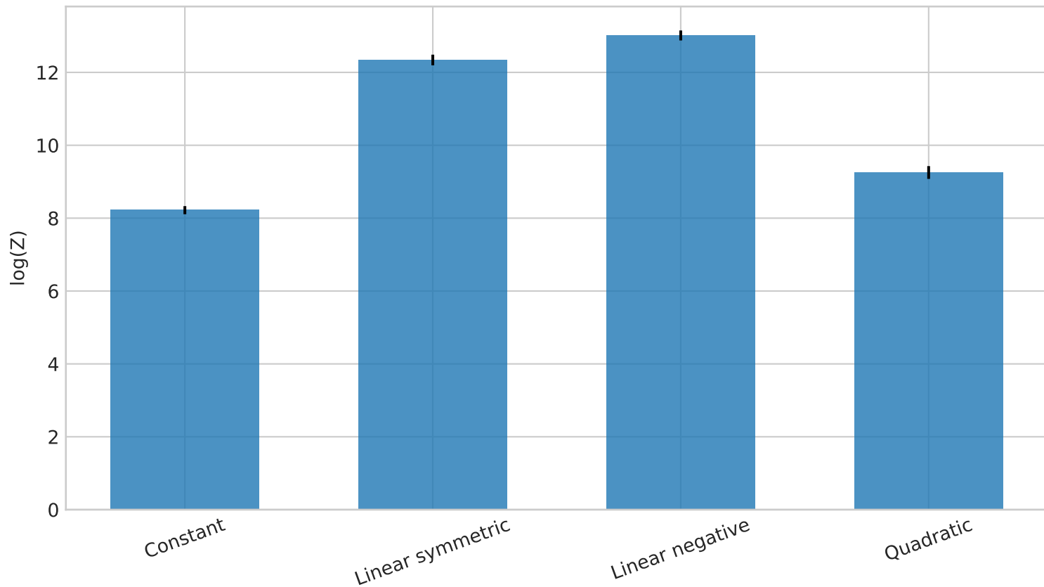
Bayesian evidence comparison (same data, different models)
