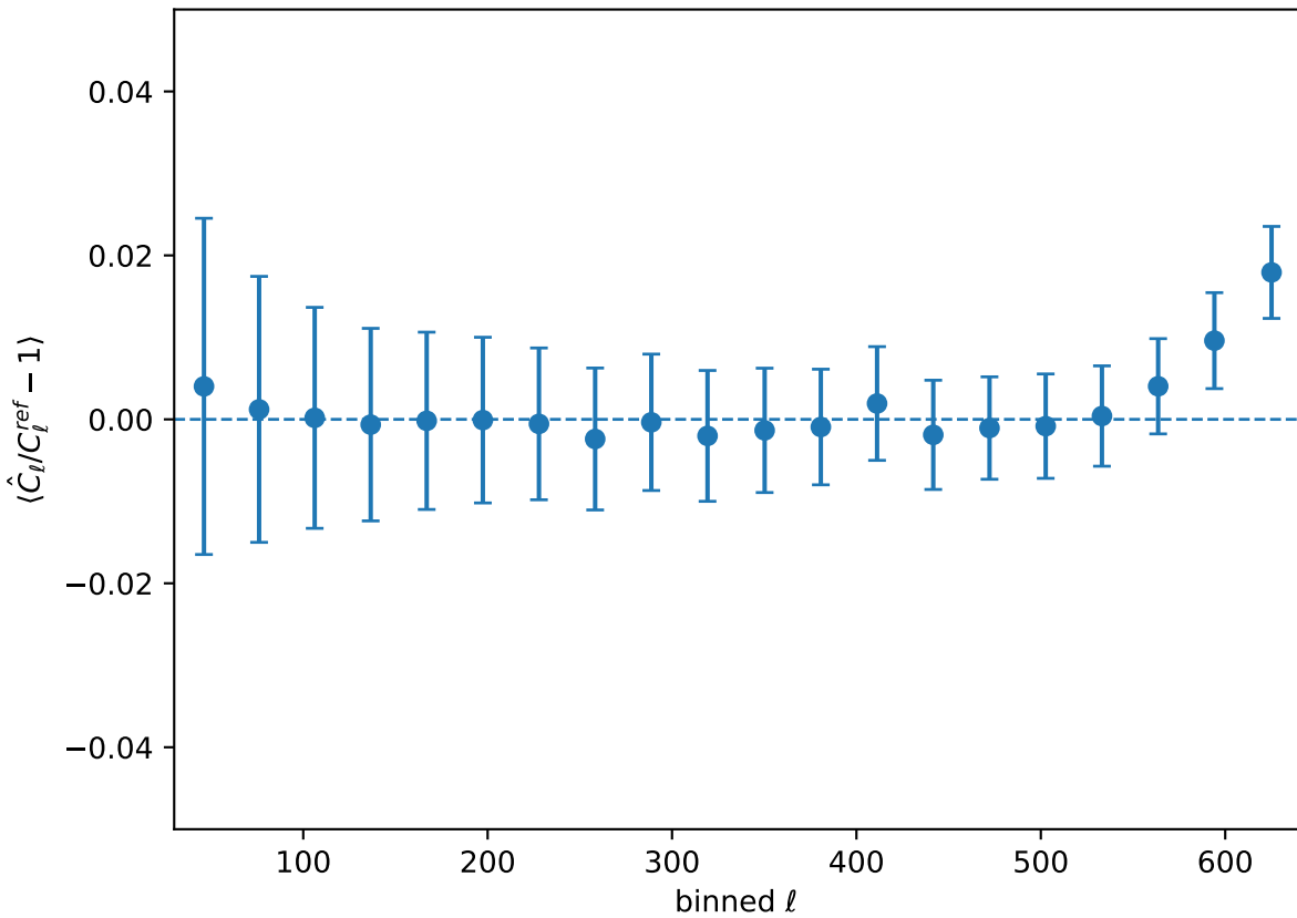
Binned relative difference (nreal=50)
