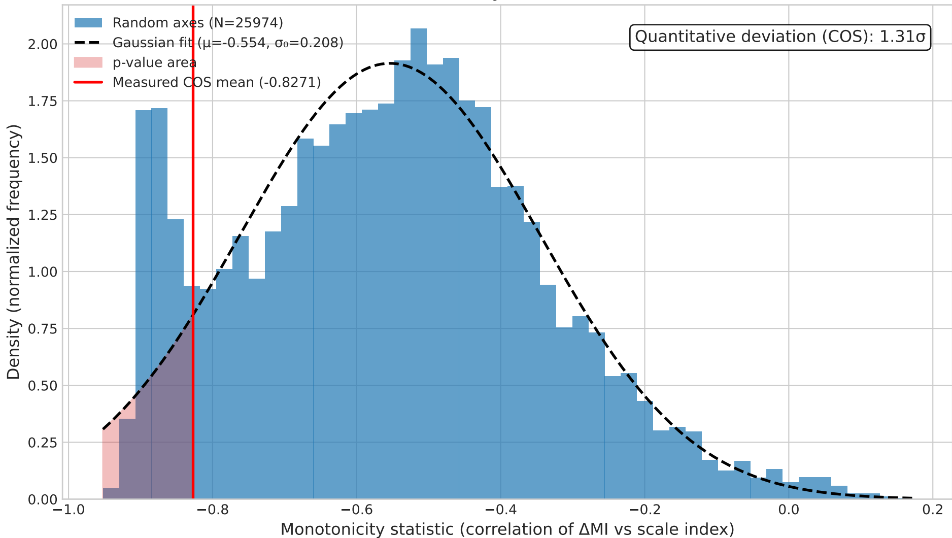
Distribution of \Delta MI monotonicity: \Lambda CDM random axes vs COS axis
