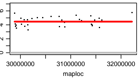
Chromosome CAXWAE020000259.1
