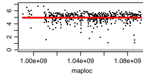
Chromosome OZ183630.2
