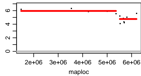
Chromosome CAXWAE020000018.1
