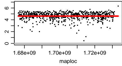
Chromosome OZ183646.2
