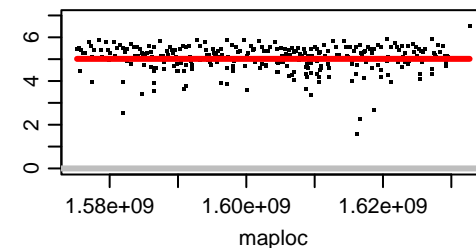
Chromosome OZ183637.2
