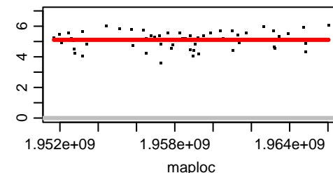
Chromosome OZ183645.2
