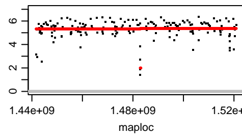
Chromosome OZ183642.2
