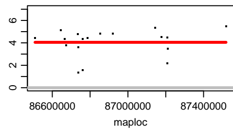
Chromosome OZ183625.2
