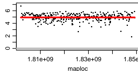
Chromosome OZ183641.2
