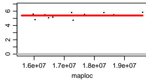
Chromosome CAXWAE020000022.1
