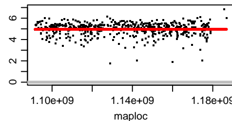
Chromosome OZ183631.2
