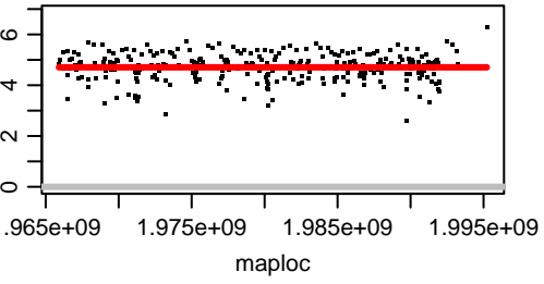
Chromosome OZ183644.2
