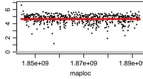
Chromosome OZ183641.2
