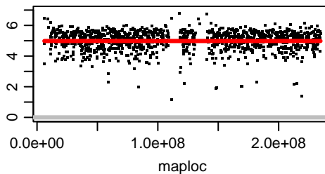
Chromosome OZ183624.2
