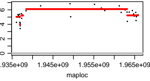
Chromosome OZ183643.2
