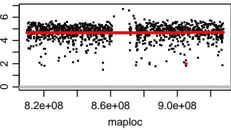
Chromosome OZ183636.2
