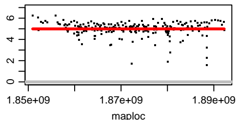
Chromosome OZ183642.2
