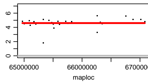
Chromosome CAXWAE020000049.1
