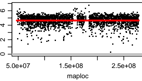
Chromosome OZ183632.2
