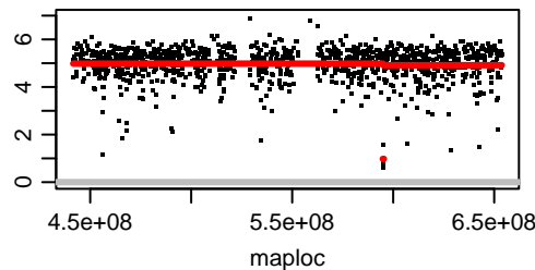
Chromosome OZ183626.2
