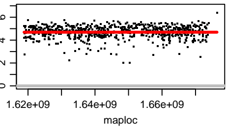
Chromosome OZ183645.2
