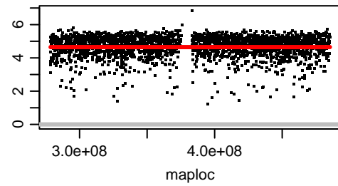
Chromosome OZ183633.2
