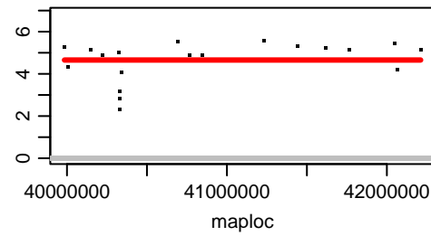
Chromosome OZ183625.2
