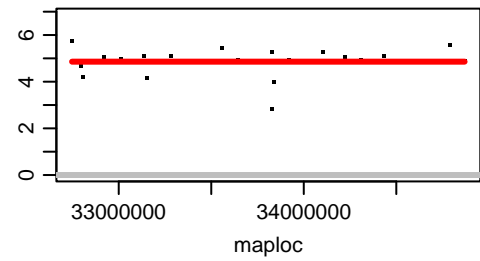
Chromosome CAXWAE020000363.1
