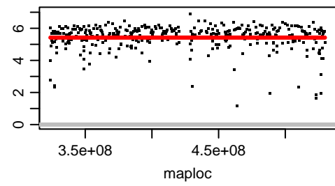
Chromosome OZ183633.2
