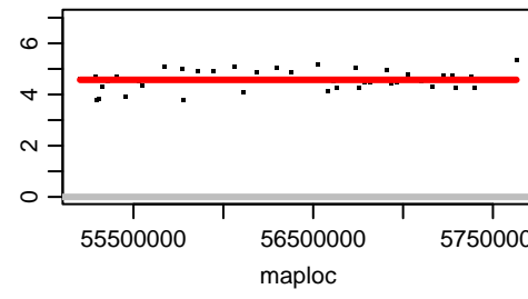
Chromosome CAXWAE020000034.1
