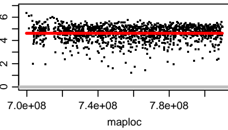
Chromosome OZ183635.2
