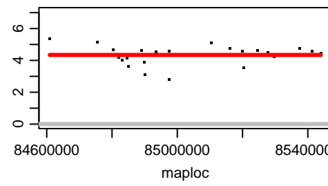
Chromosome CAXWAE020000226.1
