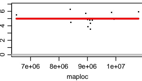
Chromosome CAXWAE020000020.1
