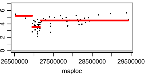
Chromosome CAXWAE020000084.1
