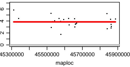
Chromosome OZ183627.2
