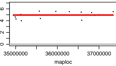
Chromosome CAXWAE020000409.1
