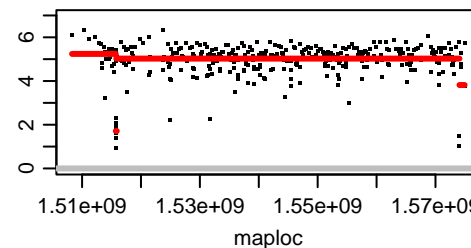
Chromosome OZ183636.2
