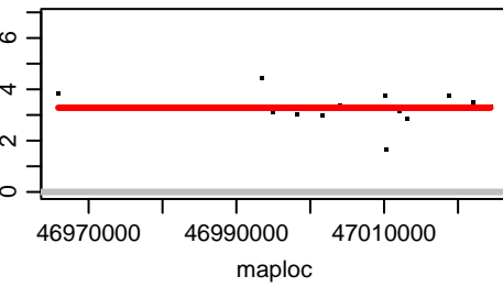
Chromosome OZ183631.2
