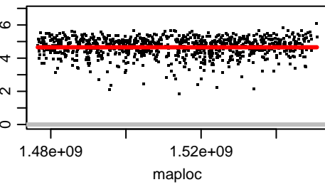
Chromosome OZ183643.2
