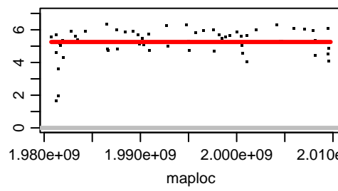
Chromosome OZ183644.2
