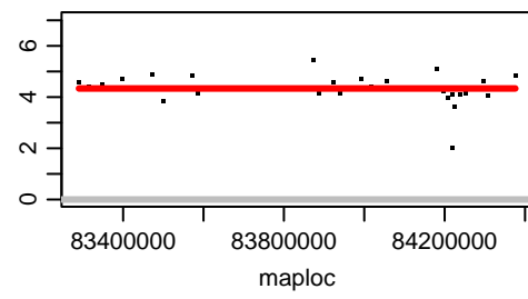
Chromosome CAXWAE020000116.1
