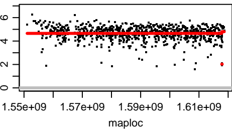
Chromosome OZ183644.2
