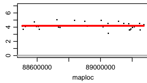
Chromosome OZ183627.2
