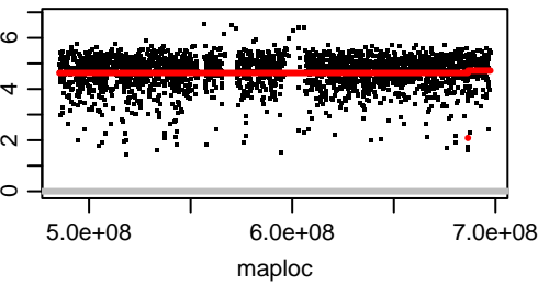
Chromosome OZ183634.2
