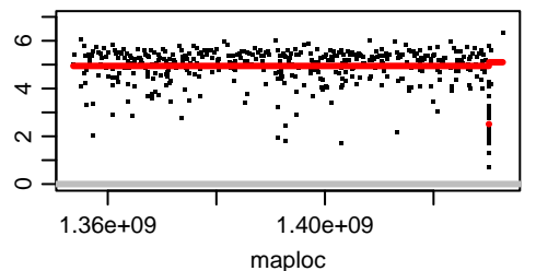
Chromosome OZ183634.2
