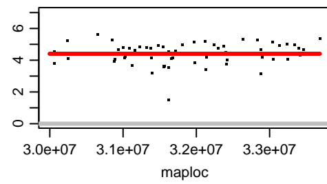
Chromosome CAXWAE020000020.1
