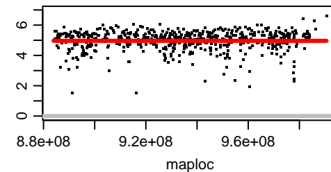
Chromosome OZ183629.2
