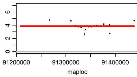
Chromosome OZ183631.2
