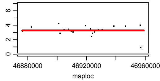
Chromosome OZ183630.2
