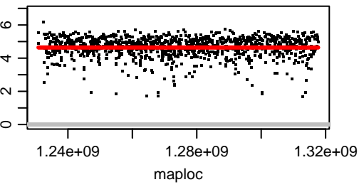
Chromosome OZ183640.2
