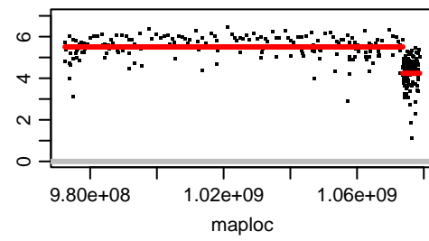
Chromosome OZ183637.2
