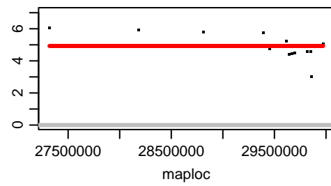
Chromosome CAXWAE020000018.1
