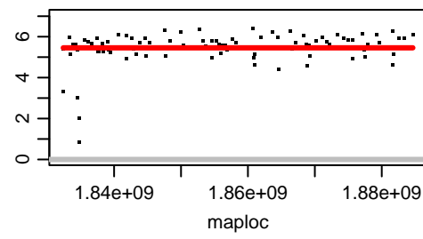
Chromosome OZ183640.2
