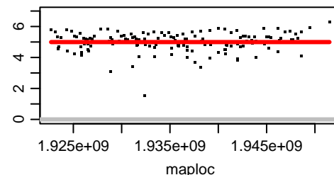
Chromosome OZ183644.2
