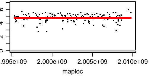
Chromosome OZ183645.2
