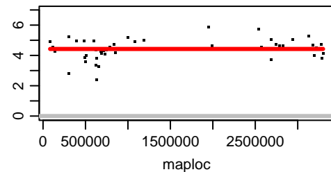
Chromosome CAXWAE020000012.1
