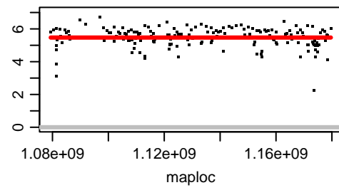
Chromosome OZ183638.2
