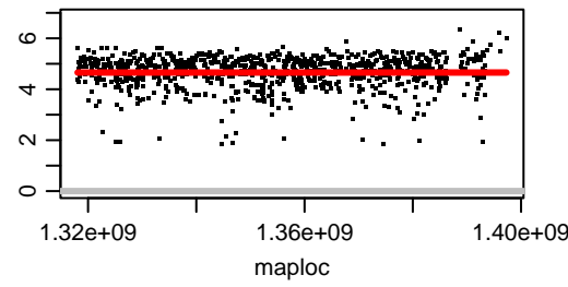
Chromosome OZ183641.2
