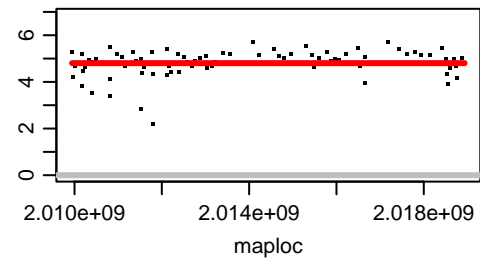
Chromosome OZ183646.2
