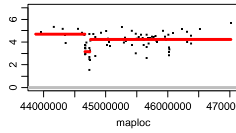
Chromosome CAXWAE020000026.1
