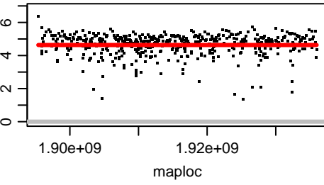
Chromosome OZ183642.2
