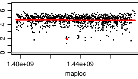
Chromosome OZ183642.2
