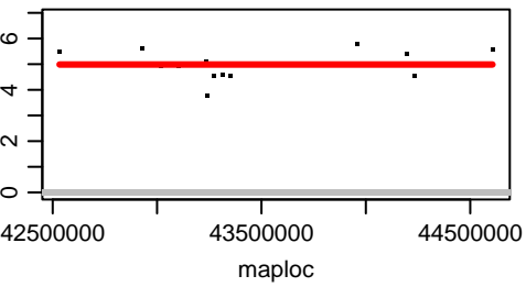
Chromosome OZ183626.2
