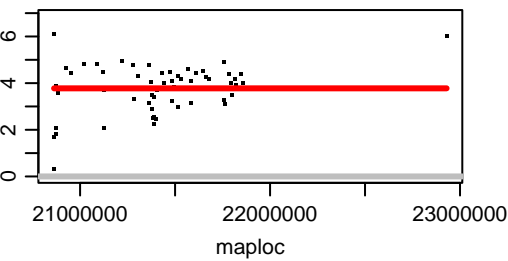
Chromosome CAXWAE020000023.1
