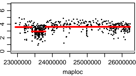
Chromosome CAXWAE020000051.1
