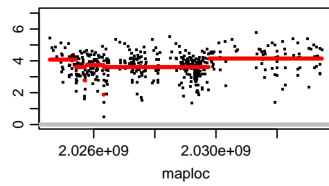
Chromosome OZ183646.2
