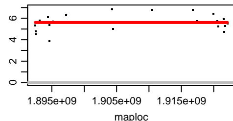
Chromosome OZ183643.2
