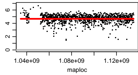
Chromosome OZ183638.2
