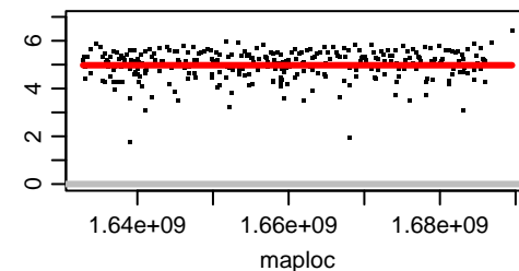
Chromosome OZ183638.2
