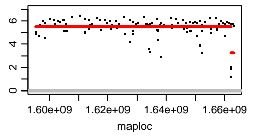
Chromosome OZ183645.2
