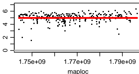
Chromosome OZ183640.2
