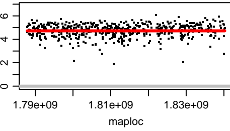
Chromosome OZ183640.2
