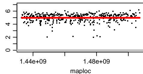
Chromosome OZ183635.2
