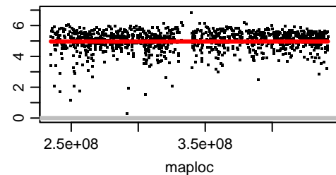
Chromosome OZ183625.2
