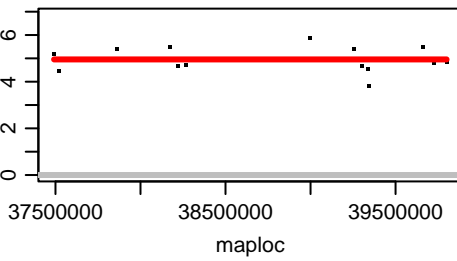
Chromosome OZ183624.2
