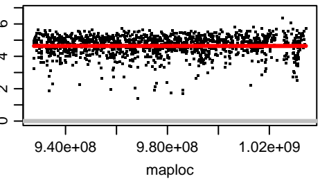
Chromosome OZ183637.2
