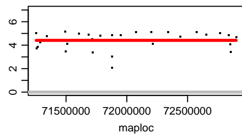
Chromosome CAXWAE020000058.1
