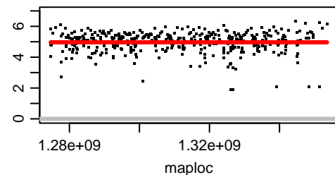
Chromosome OZ183633.2
