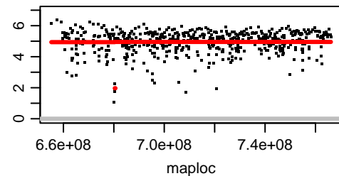
Chromosome OZ183627.2
