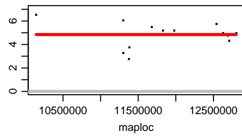
Chromosome CAXWAE020000012.1
