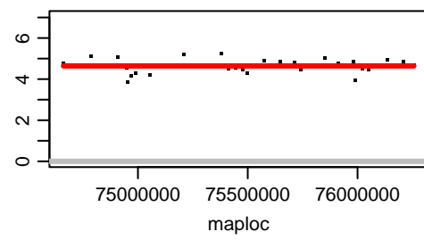
Chromosome CAXWAE020000064.1
