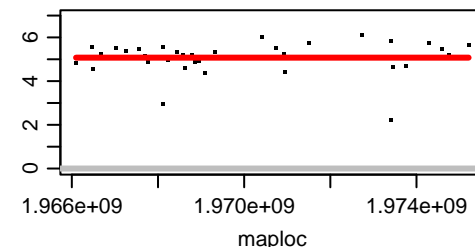
Chromosome OZ183646.2
