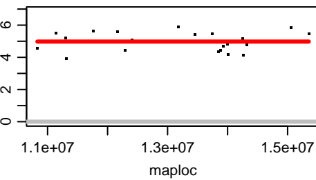
Chromosome CAXWAE020000021.1
