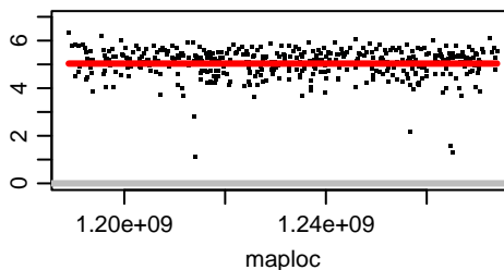
Chromosome OZ183632.2
