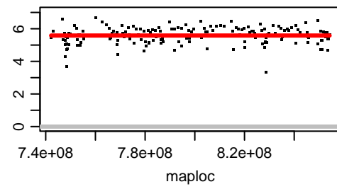
Chromosome OZ183635.2
