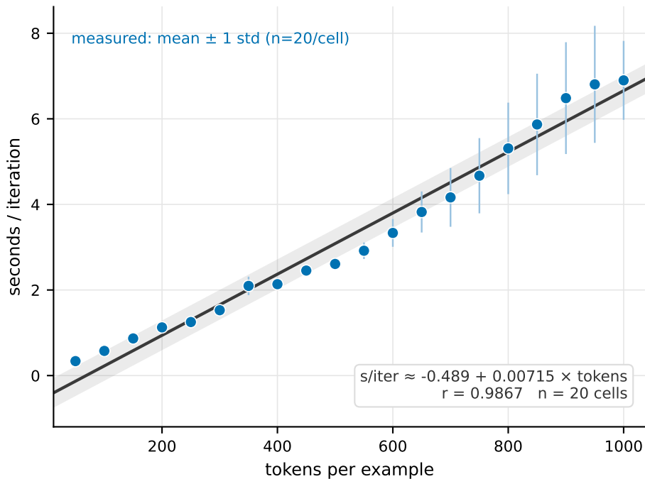
On-device LoRA training: per-iteration cost vs token count
