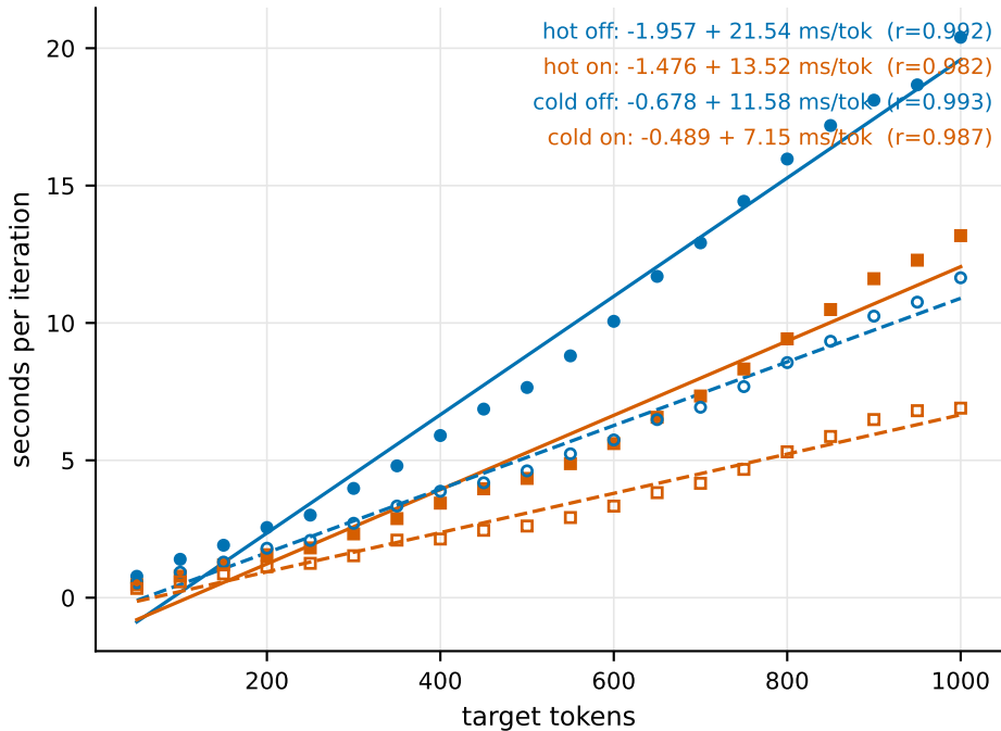
Per-iteration cost vs tokens — NAX off (blue) vs on (orange); solid = sustained-heat pass, dashed = cooled cells
