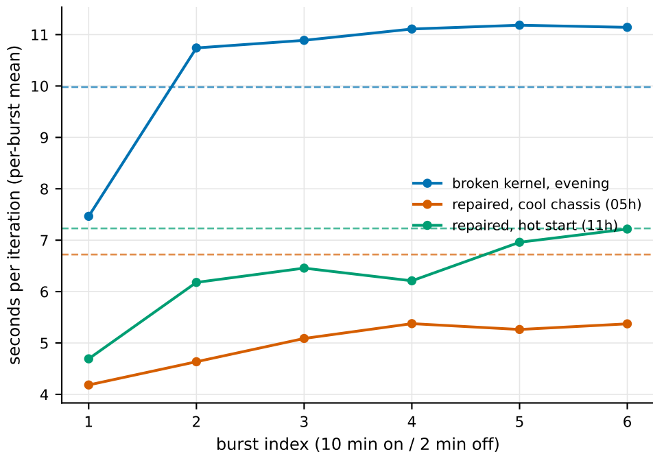
Burst-cycling vs continuous training (dashed = continuous reference)
