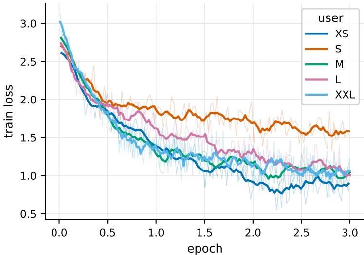
on-device User-LoRA convergence
