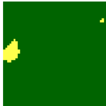
LSTM
