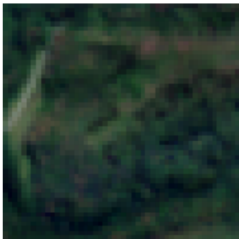
Sentinel-2 RGB
