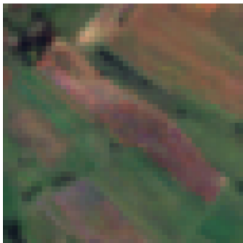
Grassland--cropland B_24.43738_46.04959
