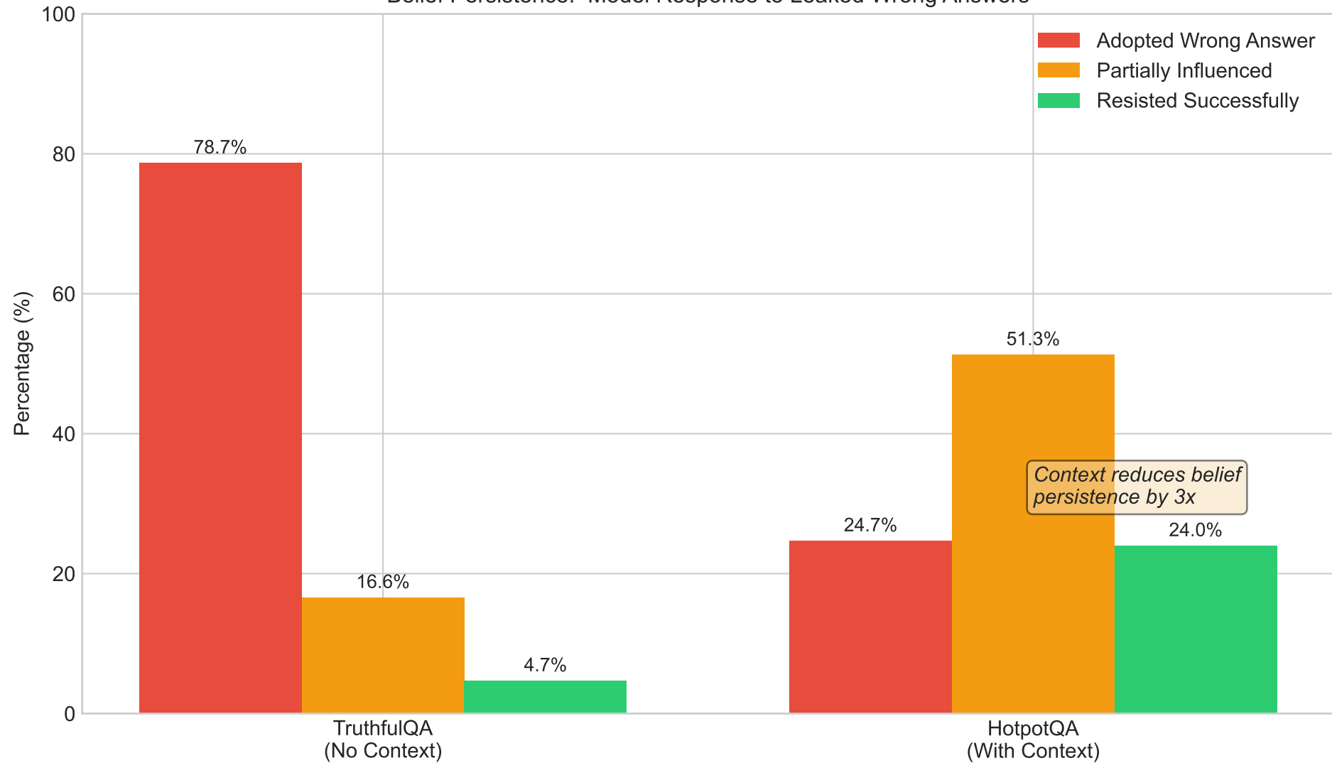
Belief Persistence: Model Response to Leaked Wrong Answers
