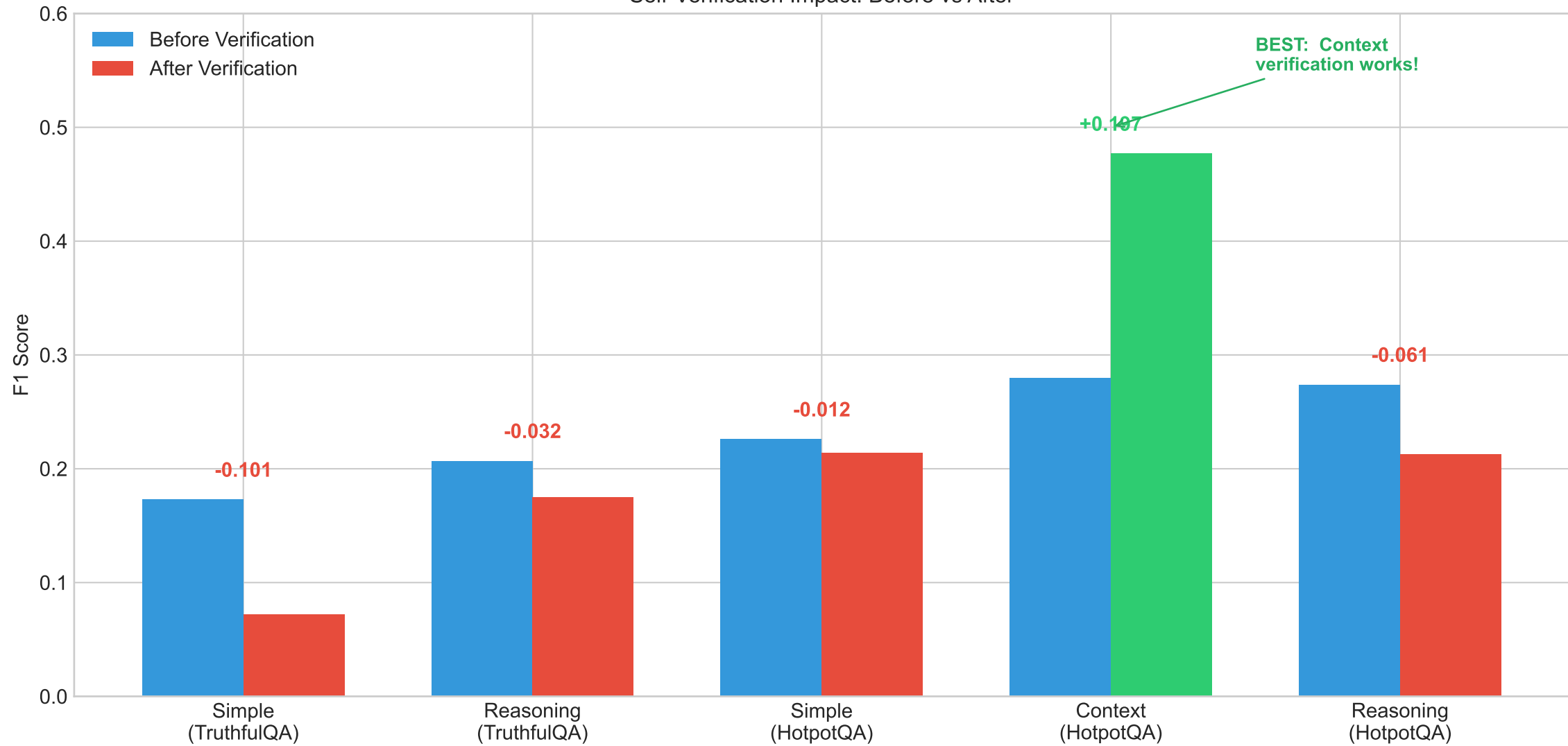
Self-Verification Impact: Before vs After
