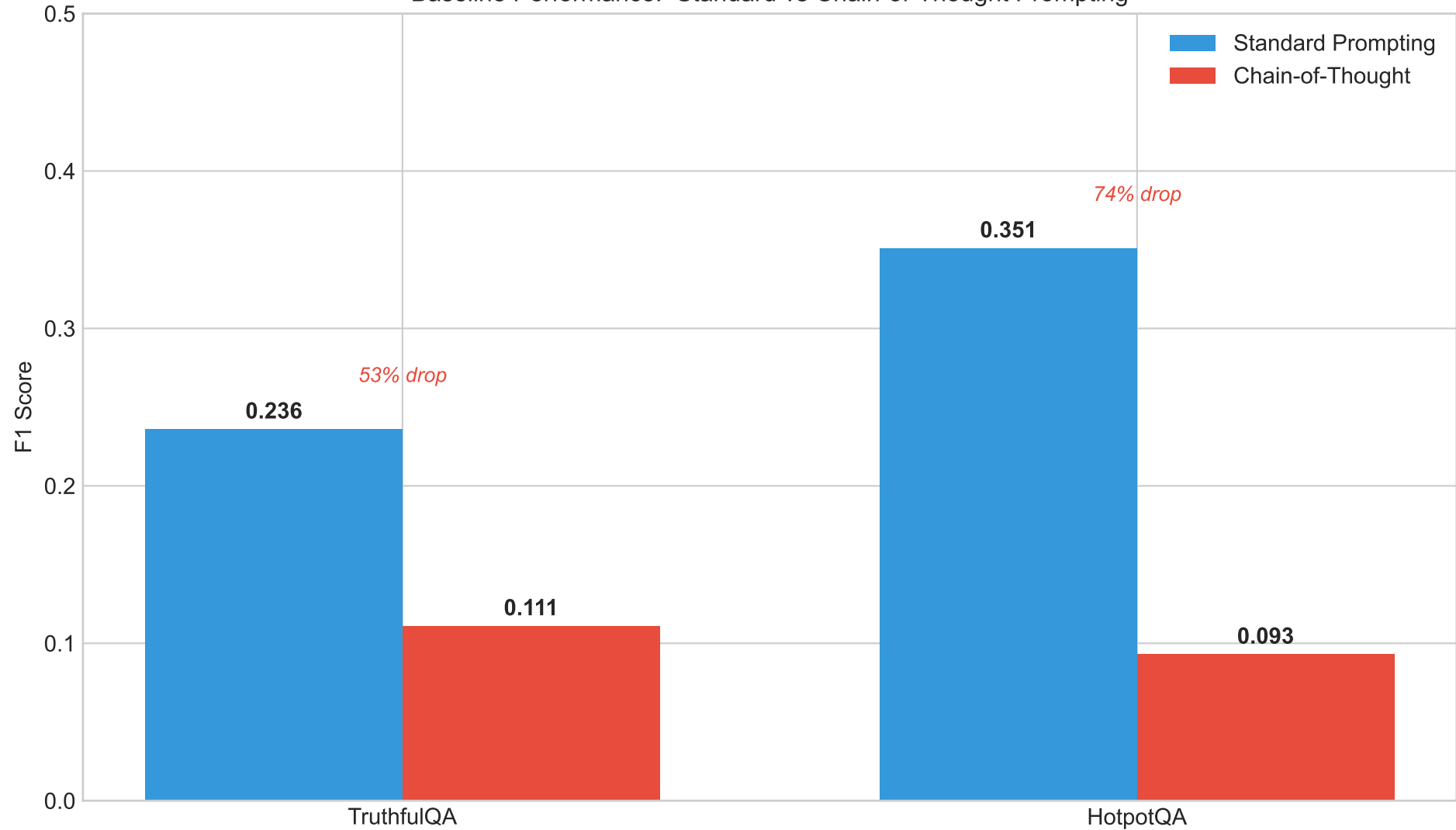
Baseline Performance: Standard vs Chain-of-Thought Prompting
