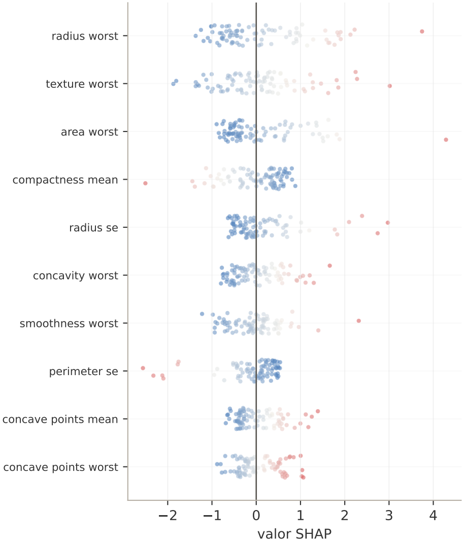
Breast Cancer
