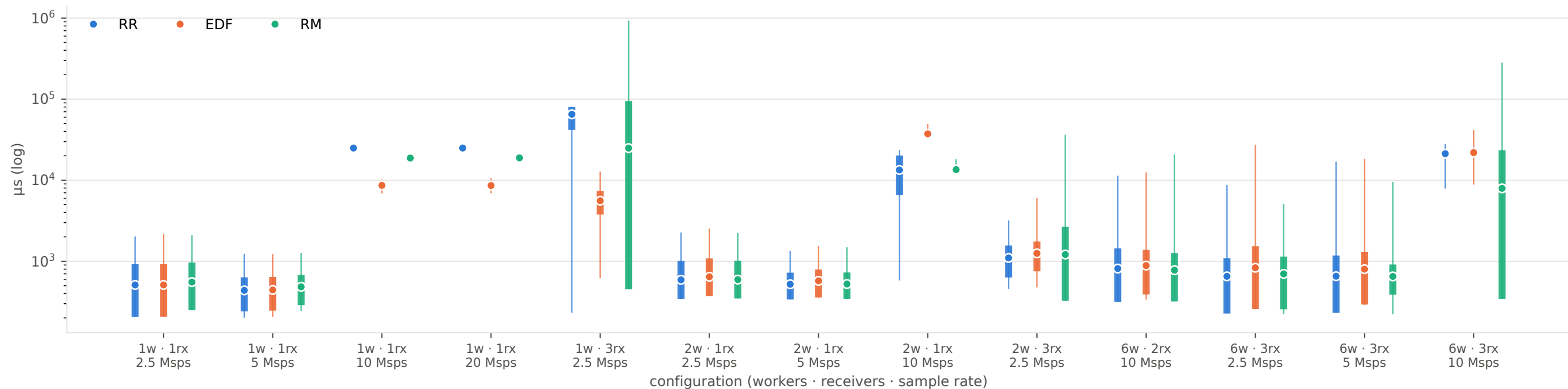
Frame response time (last sample released → decoded packet), N = 4096
