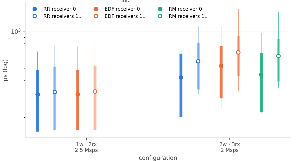
Frame response time, N = 1024, A: receiver 0 at 0.5
