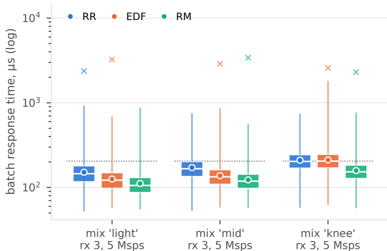
the last receiver of each mix, 5 Msps (205 \mu s period)
