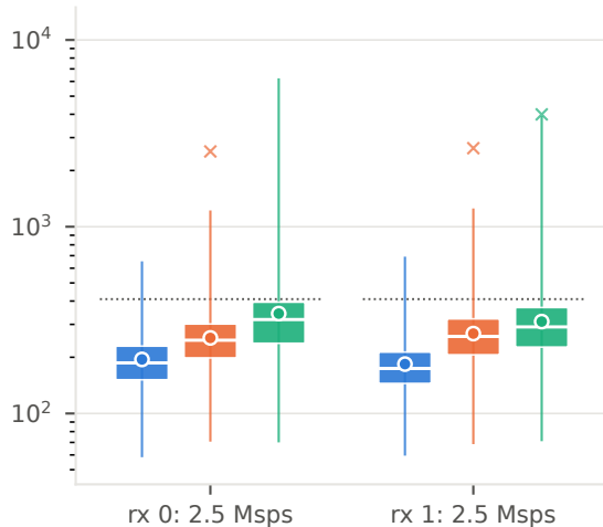
slow receivers, mix 'knee' (410 \mu s)
