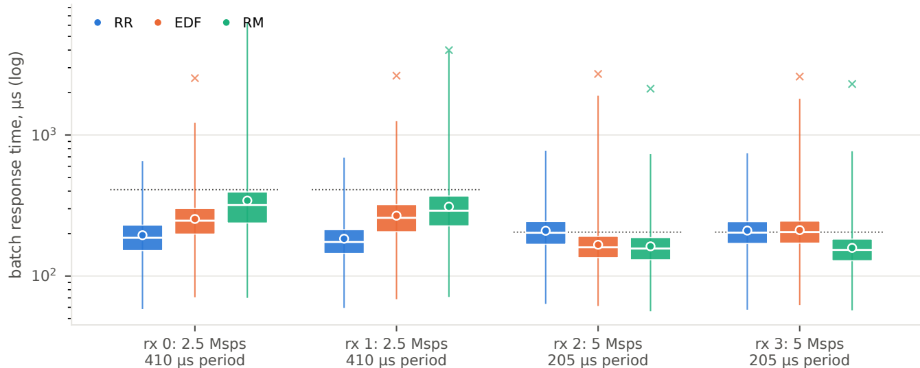
Batch response time, mix 'knee', 4 workers, N = 1024, receivers in graph order (fastest last)
