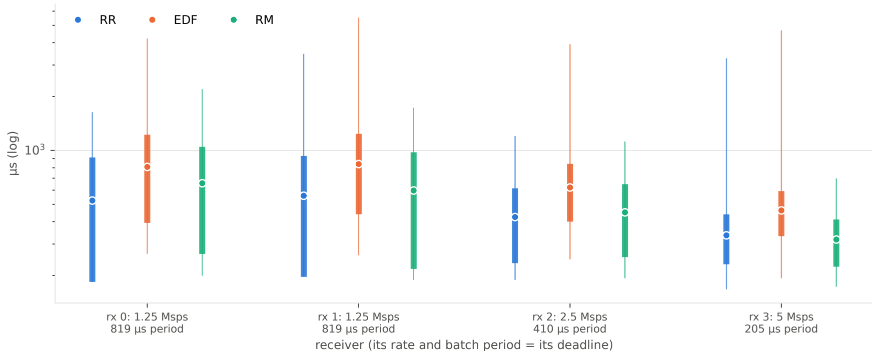
Frame response time, mix 'light', 4 workers, N = 1024, receivers in graph order (rx 3 last)
