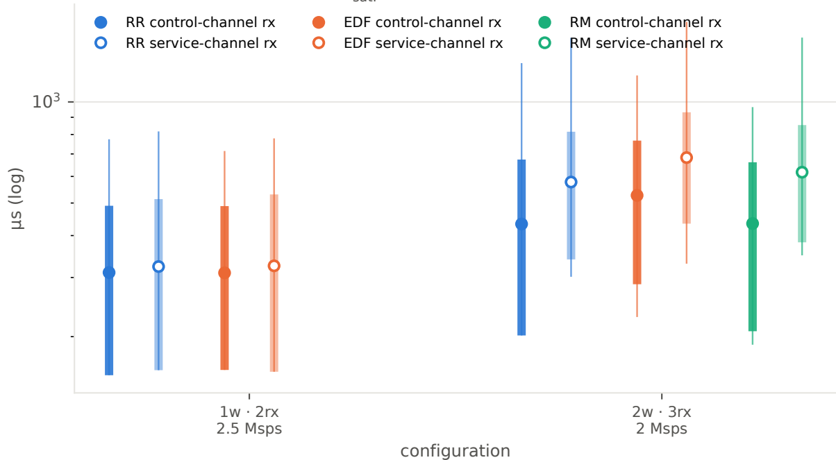
Frame response time, N = 1024, A: control-channel receiver first in graph order, at 0 sat.
