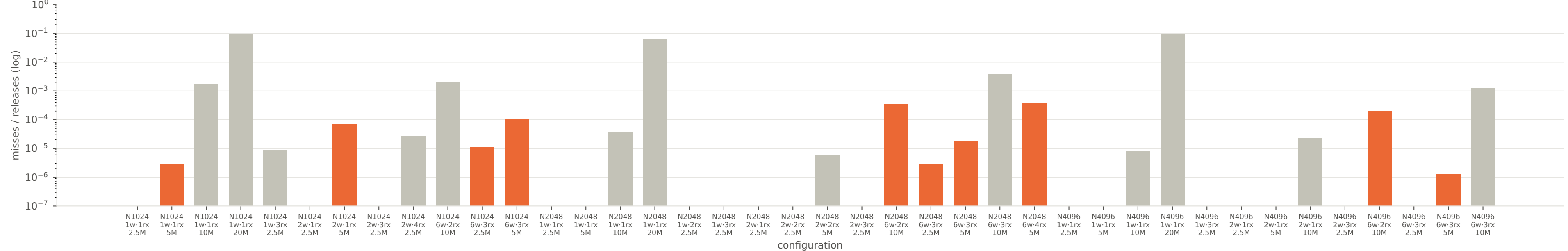
EDF: pipeline deadline-miss ratio per configuration (grey = saturated; floor of the axis = no miss)
