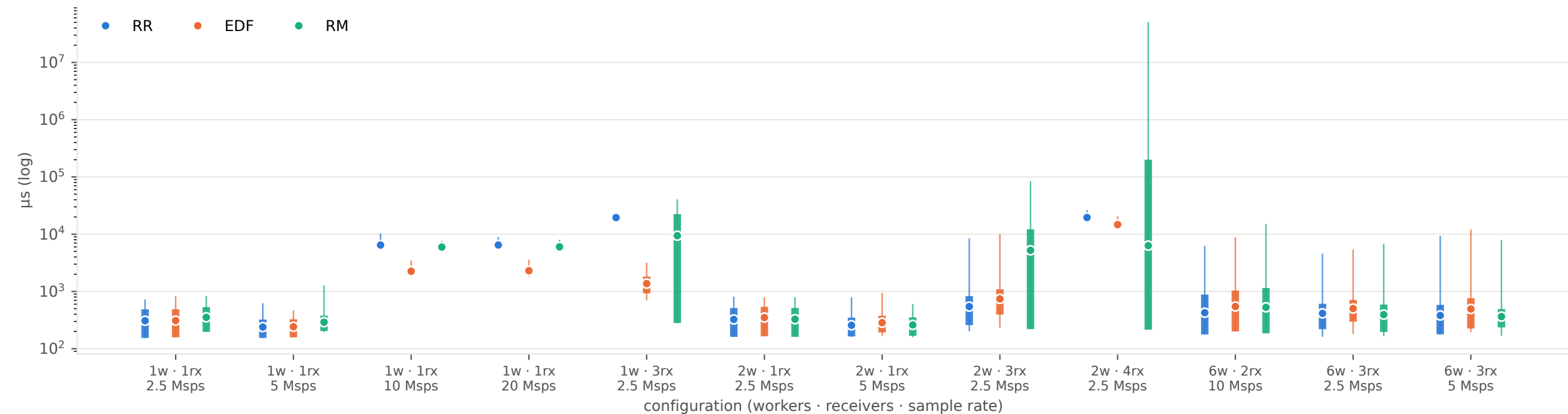
Frame response time (last sample released → decoded packet), N = 1024
