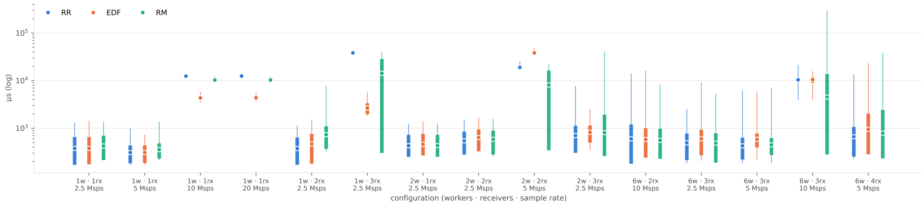
Frame response time (last sample released → decoded packet), N = 2048
