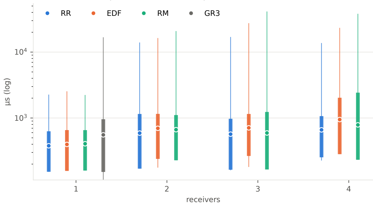
Frame response time by receiver count: GR3 (10 Msps) against the GR4 policies (unsaturated GR4 points, all N and rates pooled)
