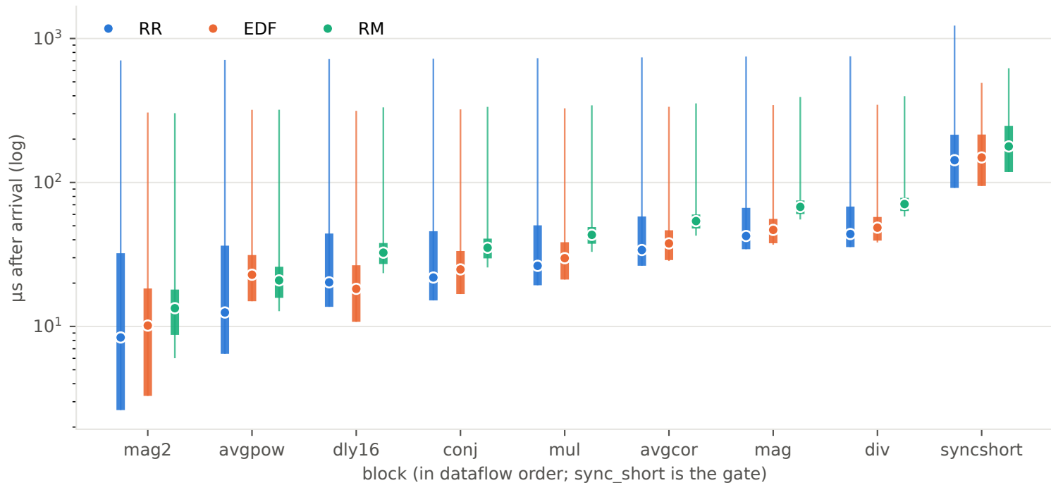
Where a batch's time goes: completion of each pre-gate block after the batch's nominal arrival, N = 2048
