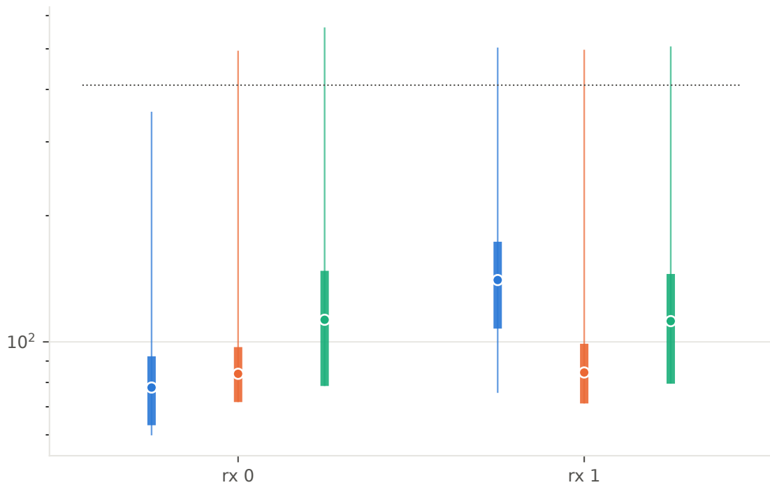
two equal receivers, two workers, 2.5 Msps each
