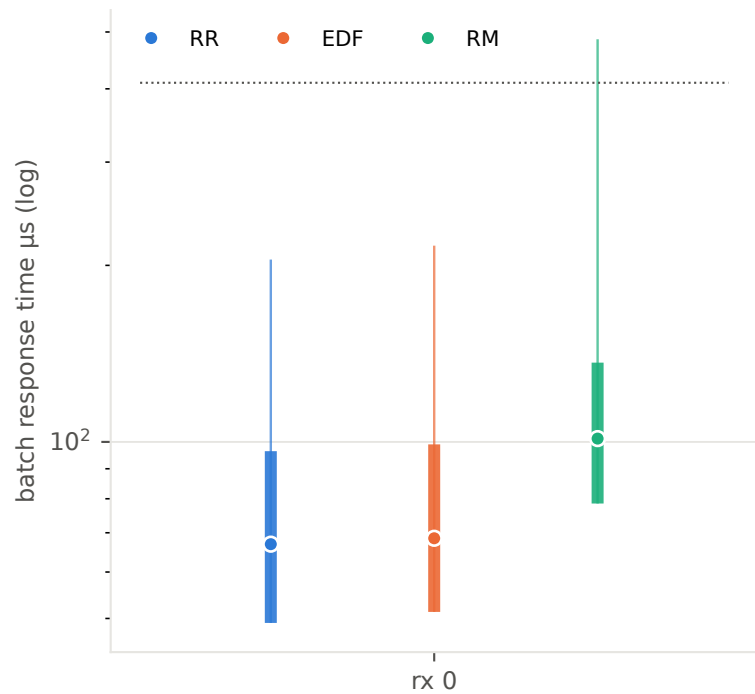
one receiver, one worker, 2.5 Msps
