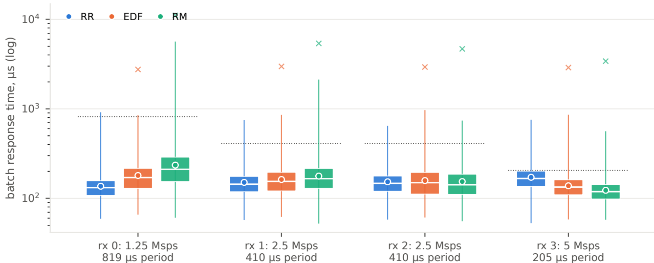
Batch response time, mix 'mid', 4 workers, N = 1024, receivers in graph order (fastest last)
