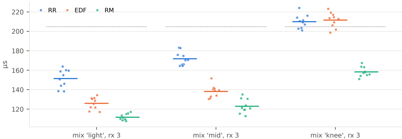
the last (5 Msps) receiver: mean batch response time of each repeat (dots) and their mean (bar)
