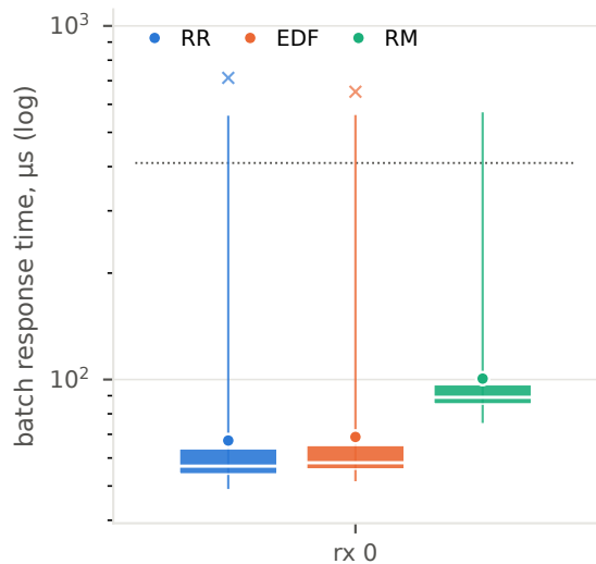
one receiver, one worker, 2.5 Msps
