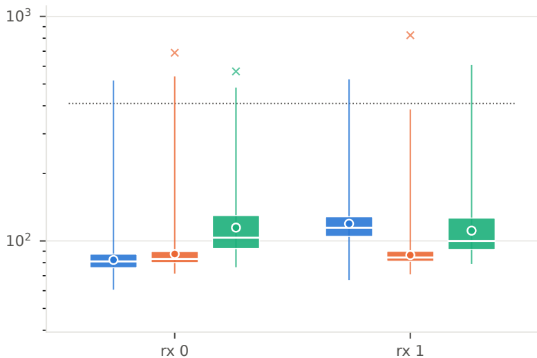
two equal receivers, two workers, 2.5 Msps each
