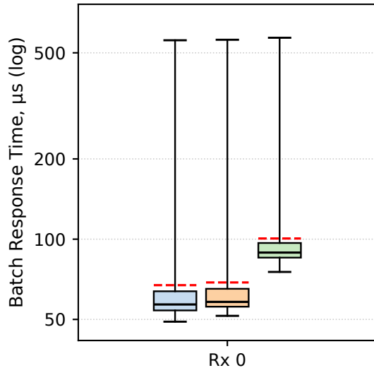
One Receiver, One Worker, 2.5 Msp/s
