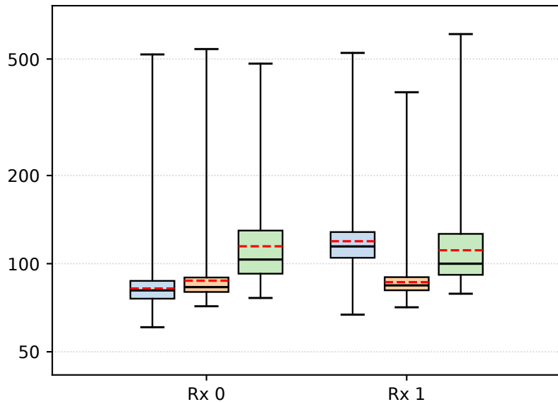
Two Equal Receivers, Two Workers, 2.5 Msp/s Each
