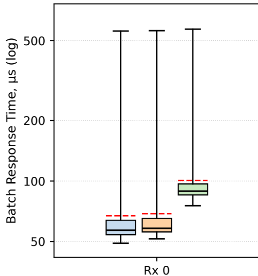
One Receiver, One Worker, 2.5 Msp/s
