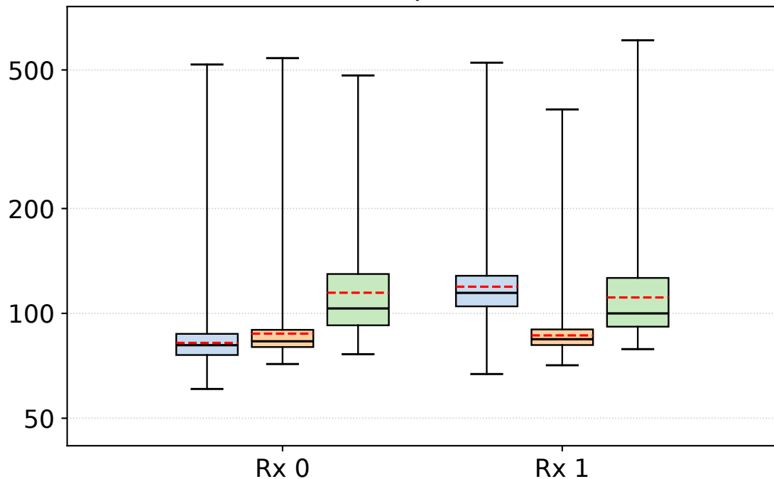
Two Equal Receivers, Two Workers, 2.5 Msps Each
