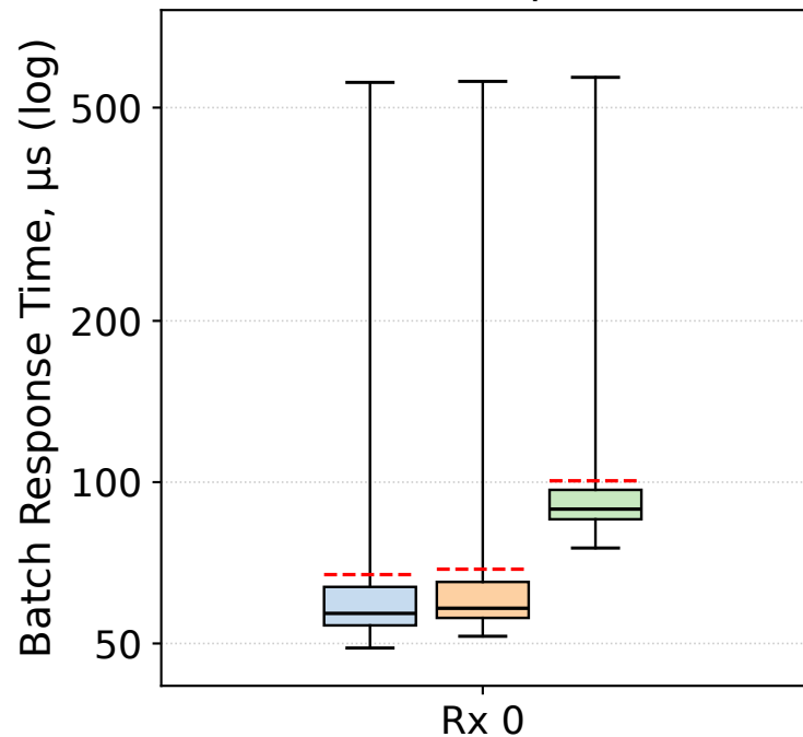
One Receiver, One Worker, 2.5 Msps
