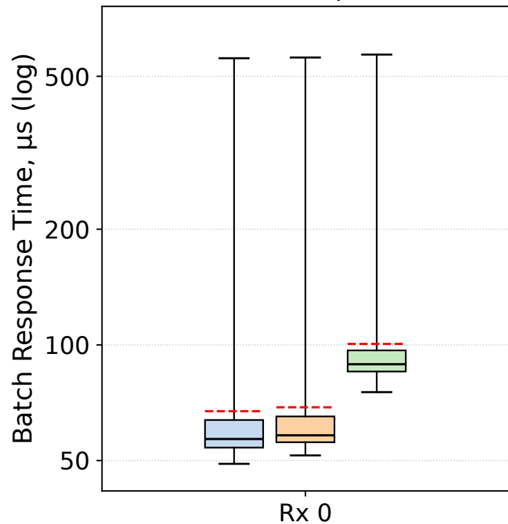
One Receiver, One Worker, 2.5 Msps
