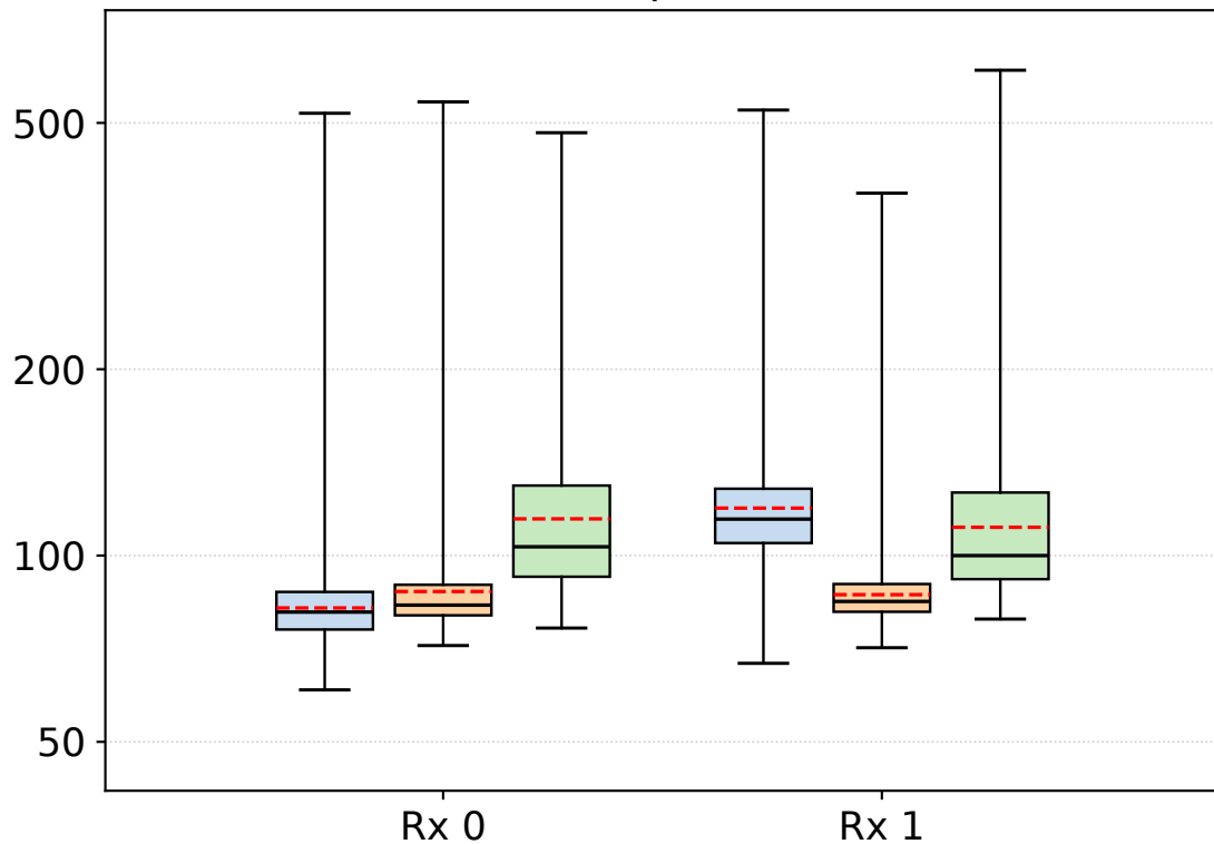
Two Equal Receivers, Two Workers, 2.5 Msps Each
