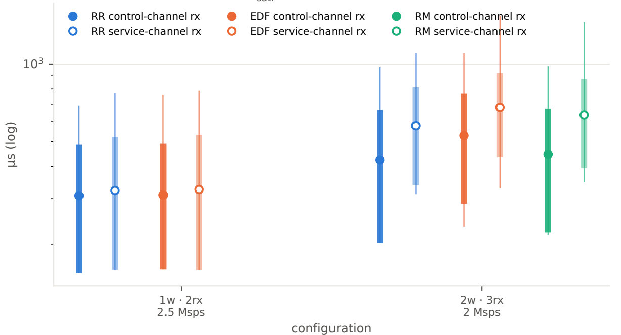
Frame response time, N = 1024, A: control-channel receiver first, at 0.5 sat.
