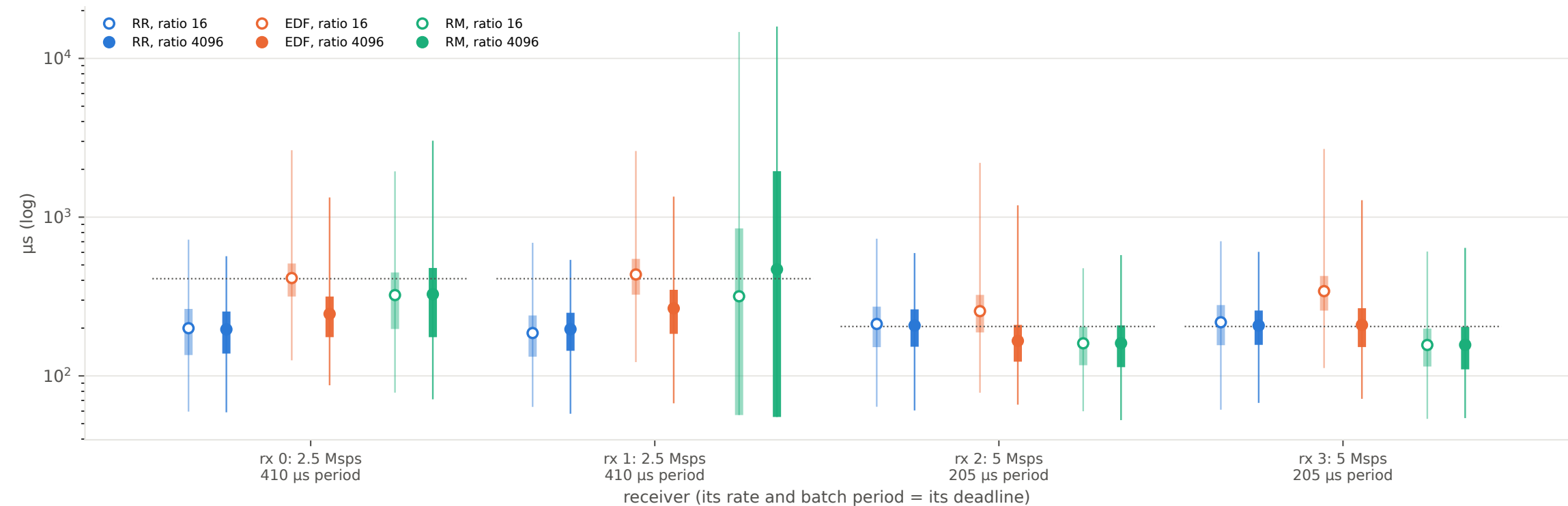
Batch response time, mix 'knee', 4 workers, N = 1024: ratio 16 (hollow) against ratio 4096 (filled)
