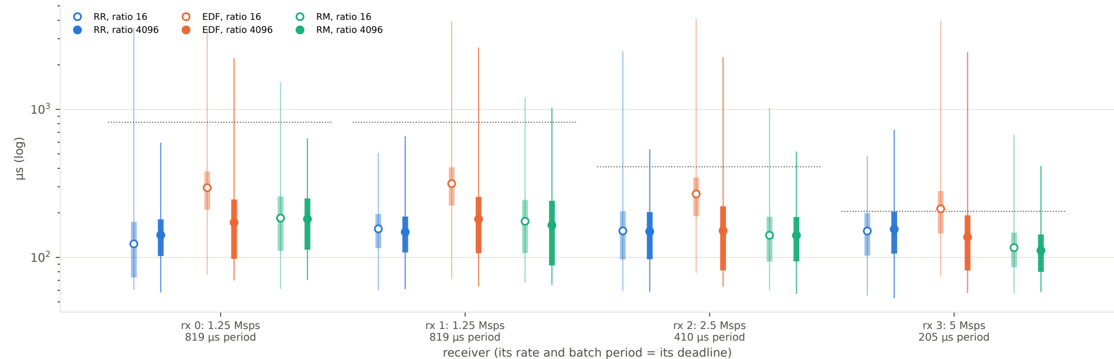
Batch response time, mix 'light', 4 workers, N = 1024: ratio 16 (hollow) against ratio 4096 (filled)
