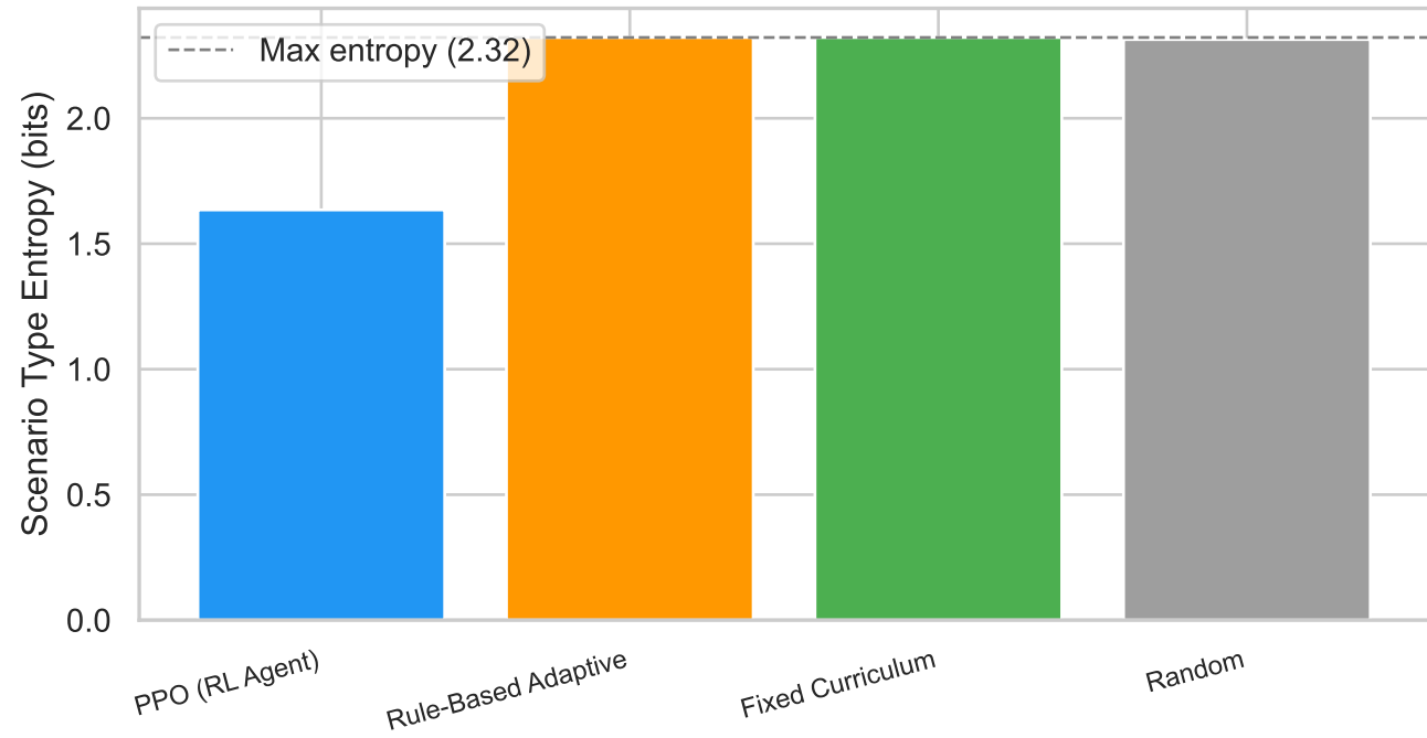
Policy Diversity: Shannon Entropy of Scenario Selection
