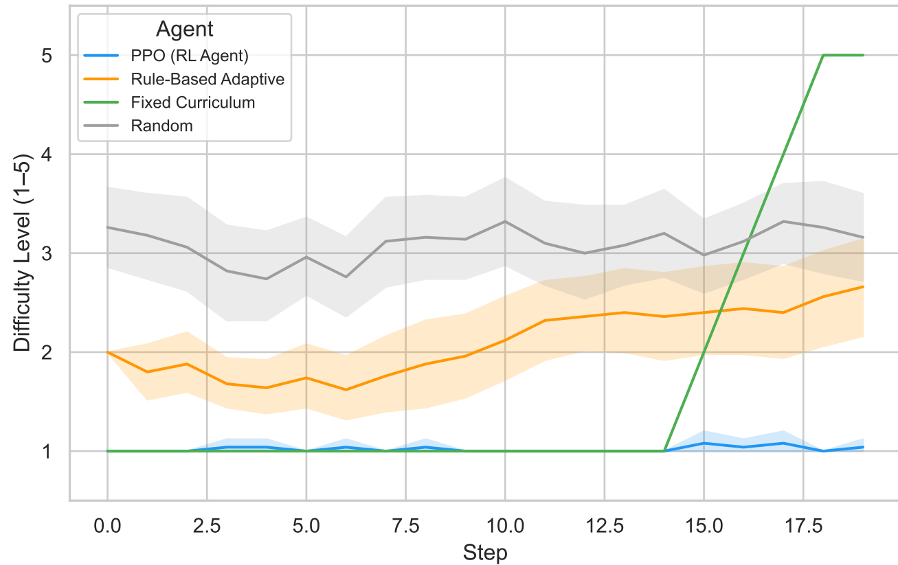
Mean Difficulty Trajectory Over Episode
