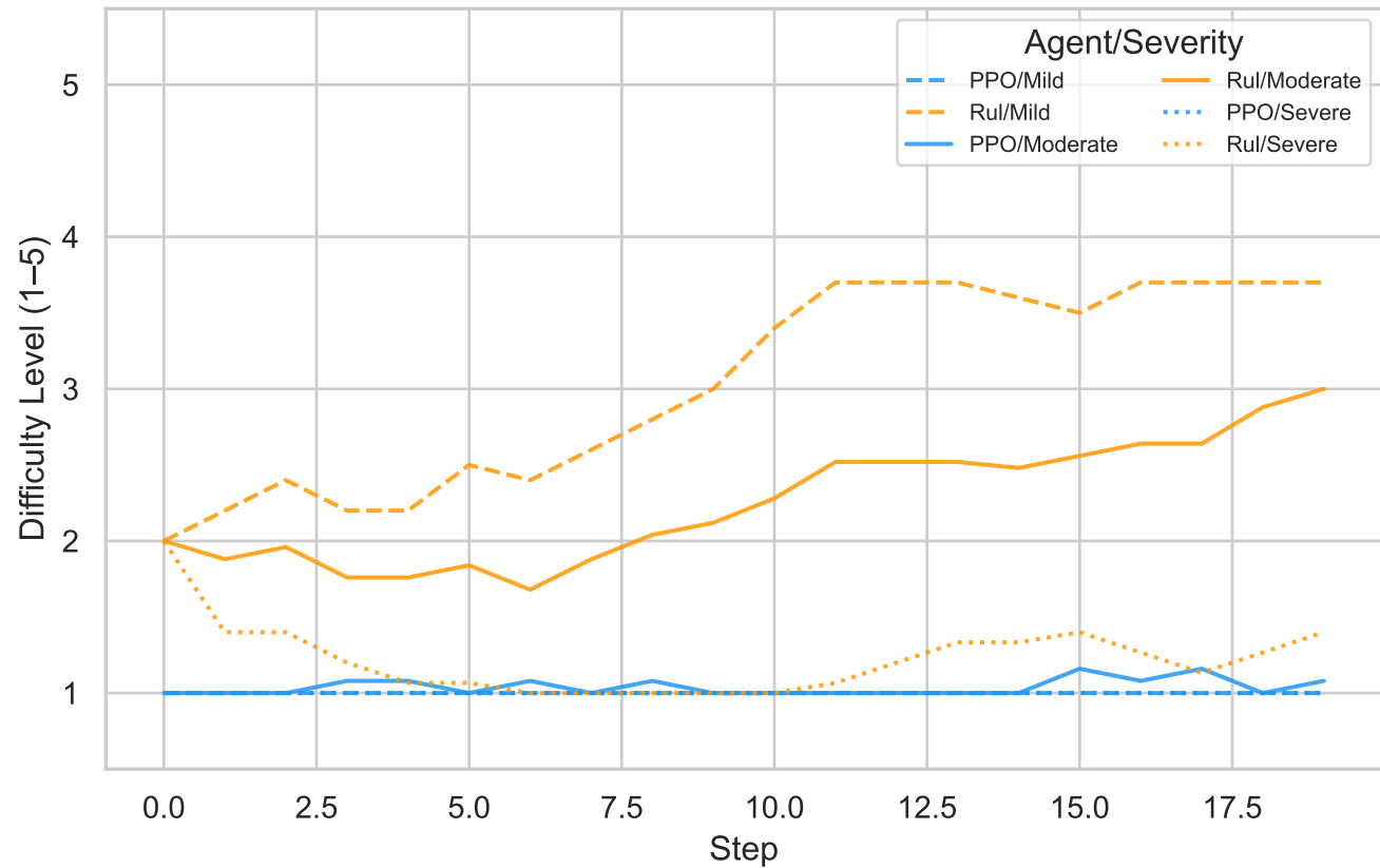
Difficulty Trajectory: PPO vs Rule-Based by ASD Severity
