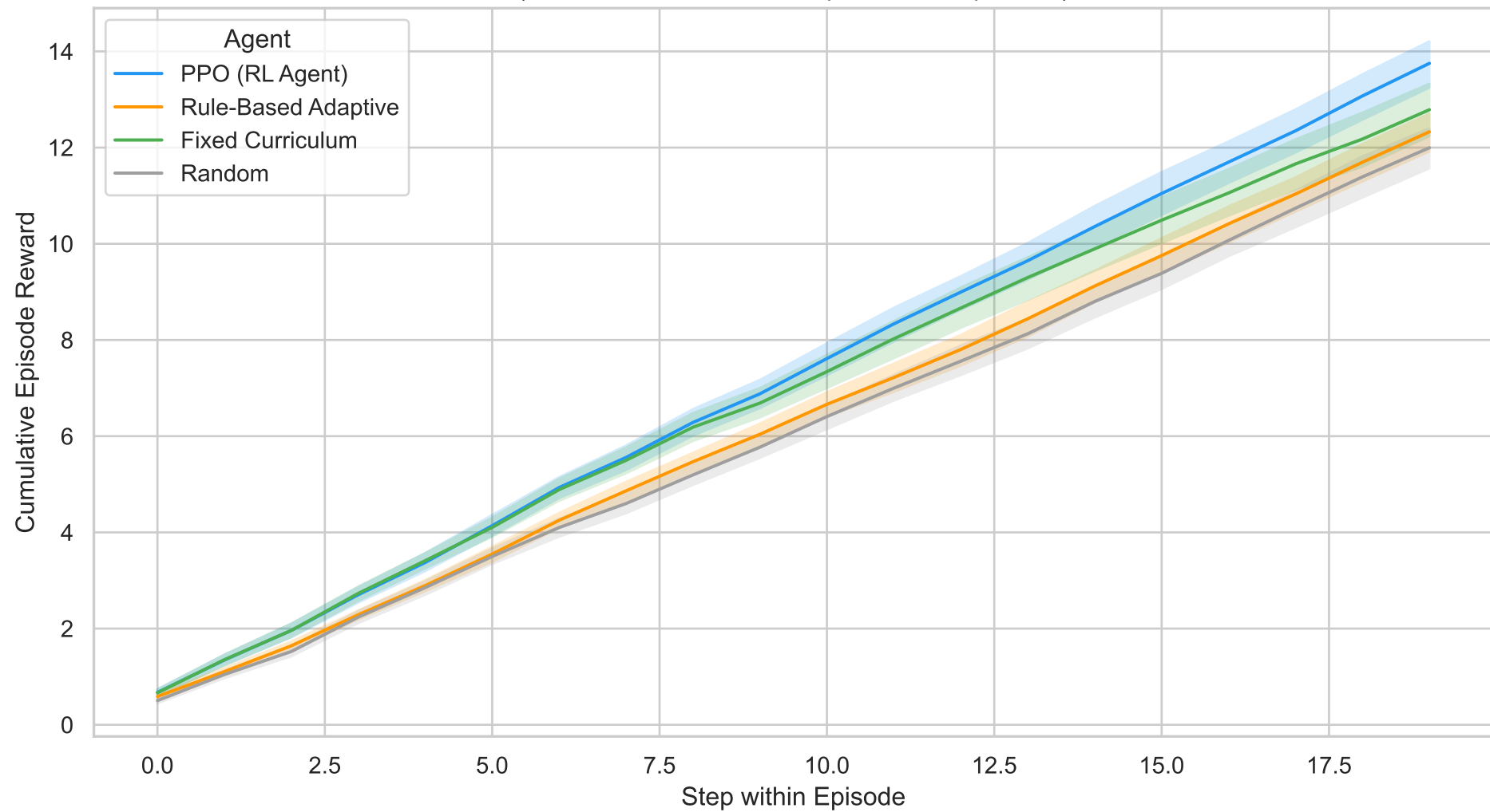
Learning Curves: Cumulative Reward over Episode Steps (mean \pm 95% CI across 10 profiles \times 5 episodes)
