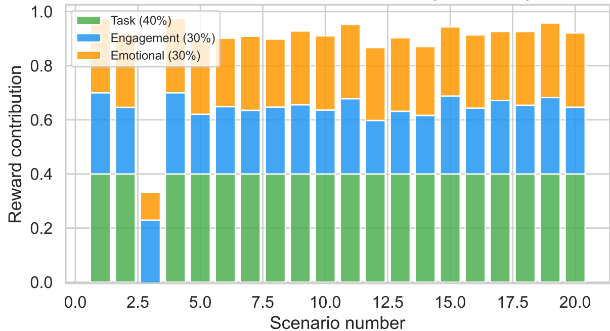
Reward Breakdown Per Scenario (40 / 30 / 30)
