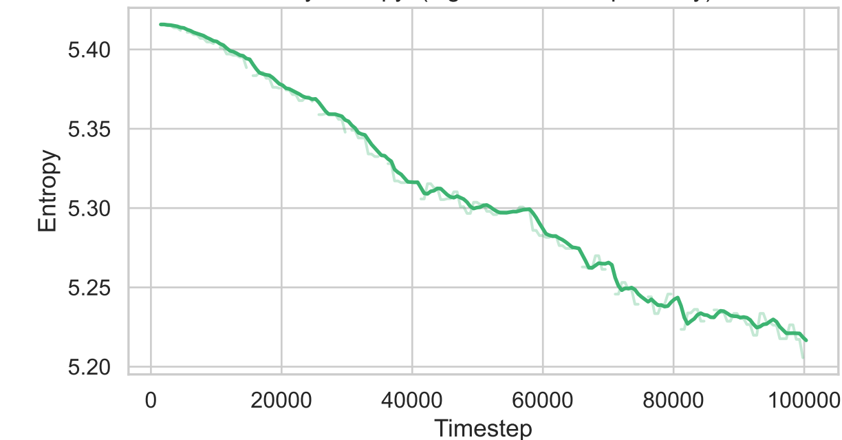
Policy Entropy (higher = more exploratory)
