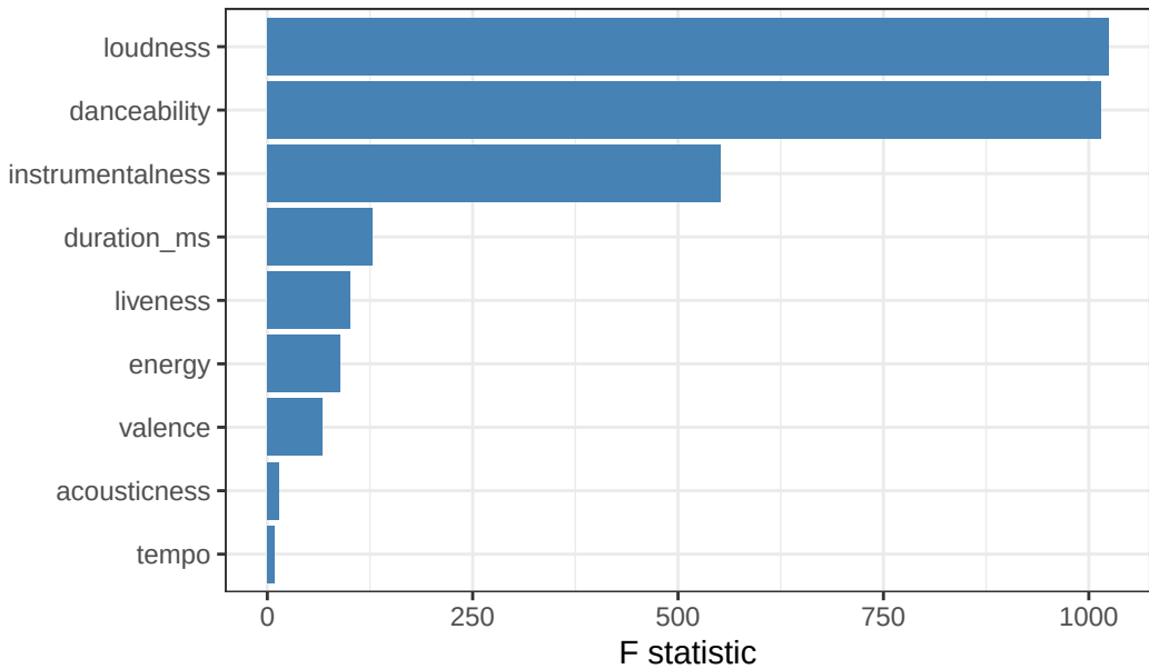
F-statistics from ANOVA table
