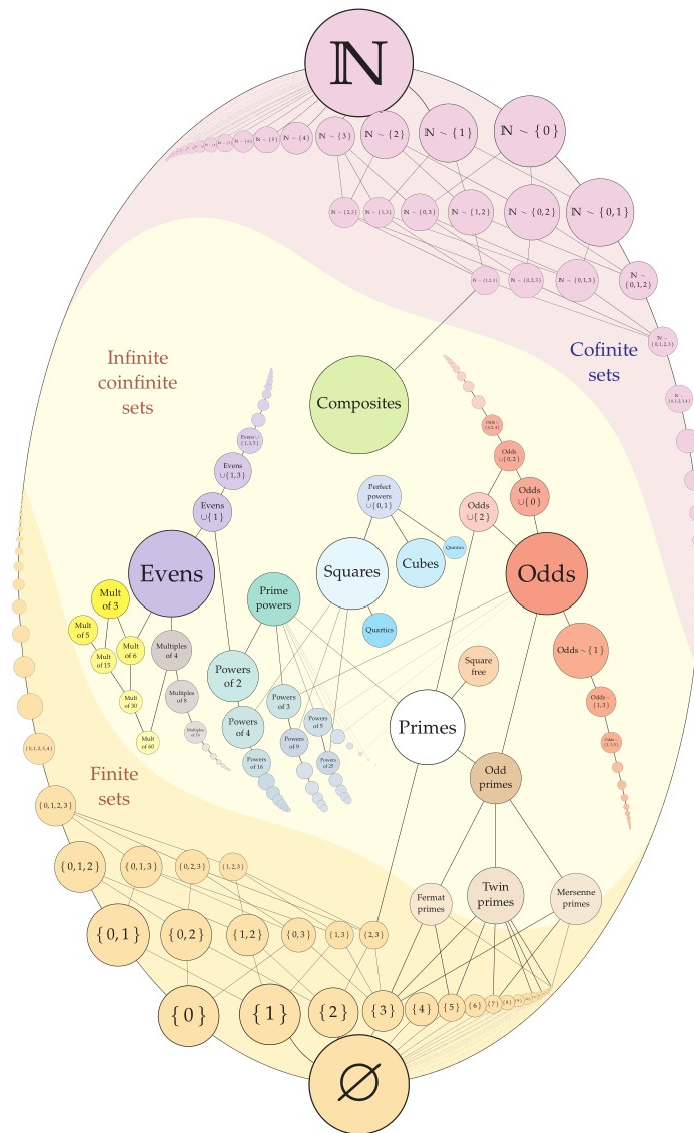
Figure 3.1 The power set lattice P(\mathbb{N}) of all sets of natural numbers, not to scale, some sets omitted...
