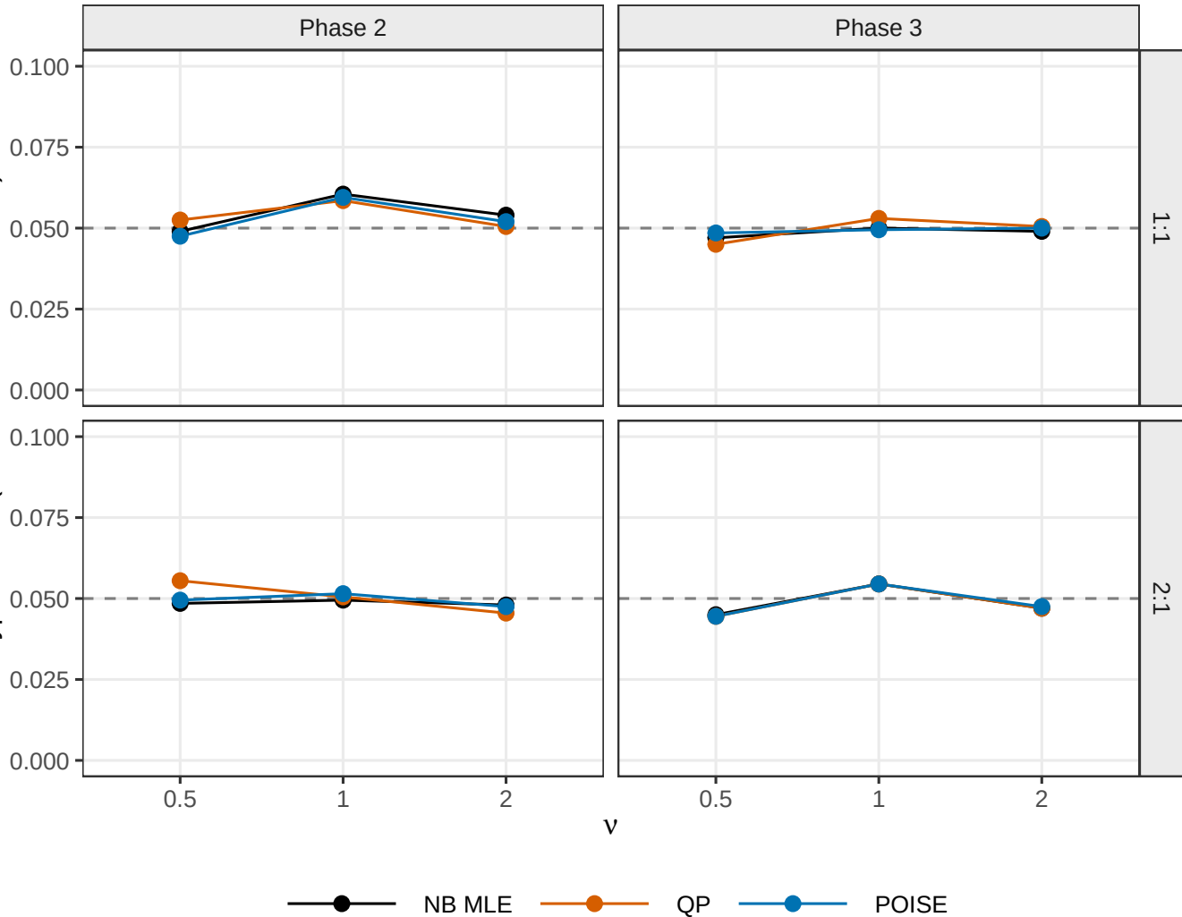
Type I error (two-sided, nominal 0.05)
